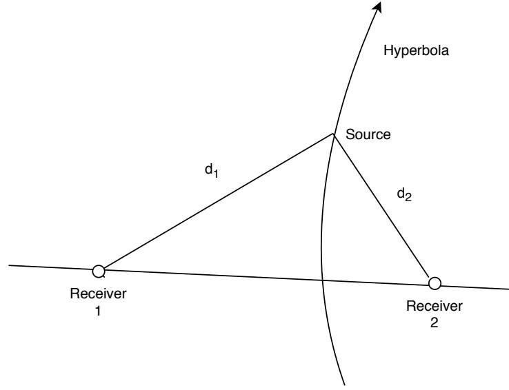
Figure 2.1: The hyperbola of a TDOA measurement
