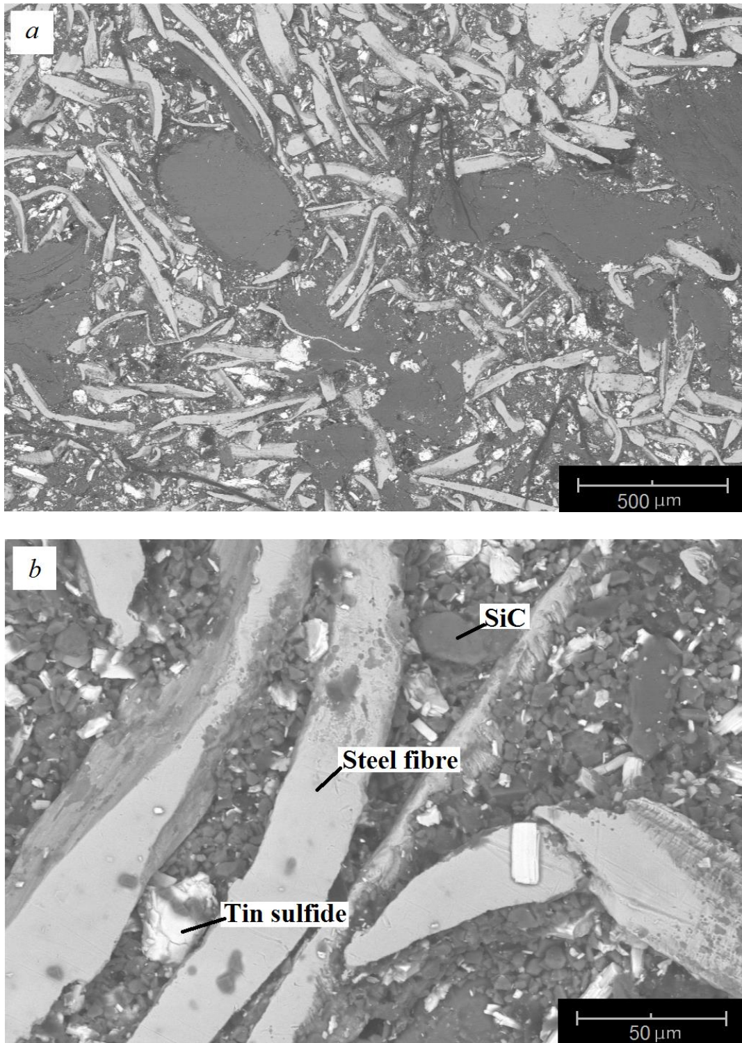
Figure 4.13. BSE images of polished surface PMSQ-WP sample at 60 ^{\circ}\text{C} at 150x (a) and 1500x (b) magnification.
