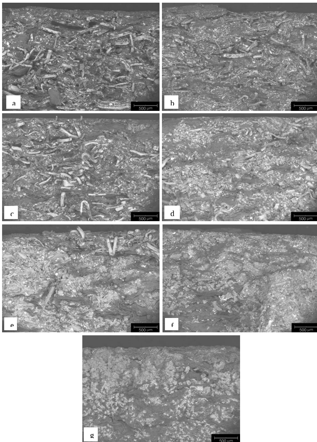
Figure 4.12. BSE images of fracture surface of PMSQ matrix composite samples in the direction of warm pressing at 100x magnification; (a) just warm pressed sample at 150 °C (PPSQ-WP), (b) just crosslinked sample after warm pressing at 300 °C (PPSQ-CL), and heat treated samples at different temperatures after crosslinking (c) PPSQ-HT400, (d) PPSQ -HT500, (e) PPSQ -HT600, (f) PPSQ -HT700, and (g) PPSQ -HT800.
