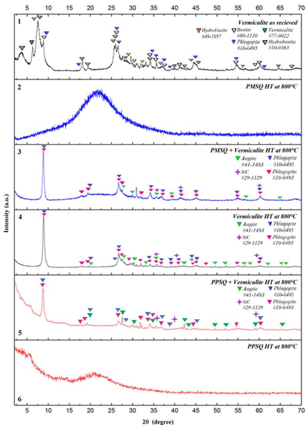
Figure 3.16. XRD pattern comparison of PMSQ-vermiculite. (1) As received vermiculite, (2) heat treated (HT) PMSQ at 800 °C, (3) PMSQ polymer + vermiculite binary mixtures heat treated at 800 °C, (4) heat treated vermiculite at 800 °C, (5) PPSQ polymer + vermiculite binary mixtures heat treated at 800 °C, and (6) heat treated PPSQ at 800 °C.
