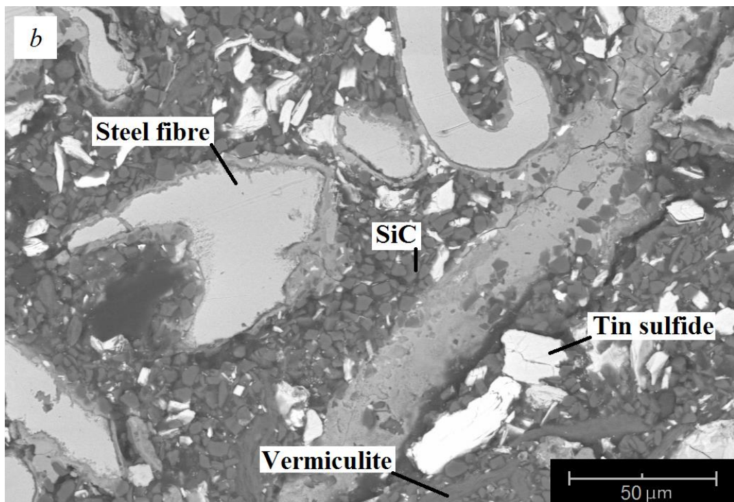
Figure 4.16. BSE images of polished surface PMSQ-HT500 sample at 150x (a) and 1500x (b) magnification.
