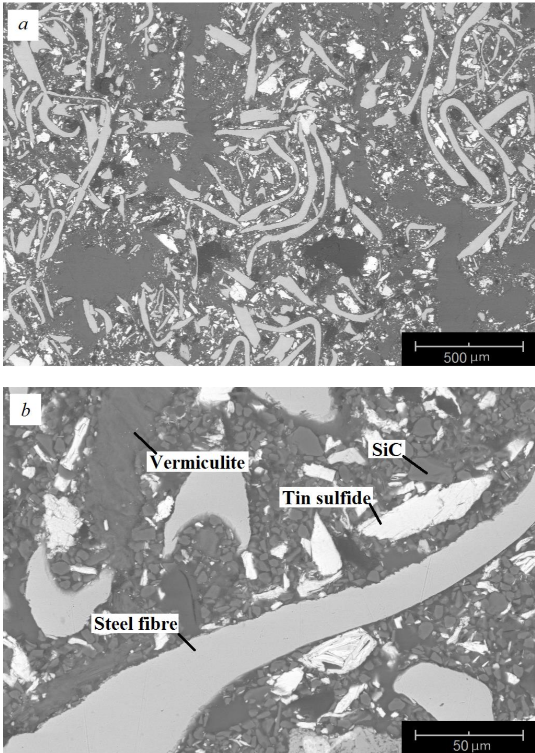
Figure 4.14. BSE images of polished surface PMSQ-CL sample at 250 °C at 150x (a) and 1500x (b) magnification.
