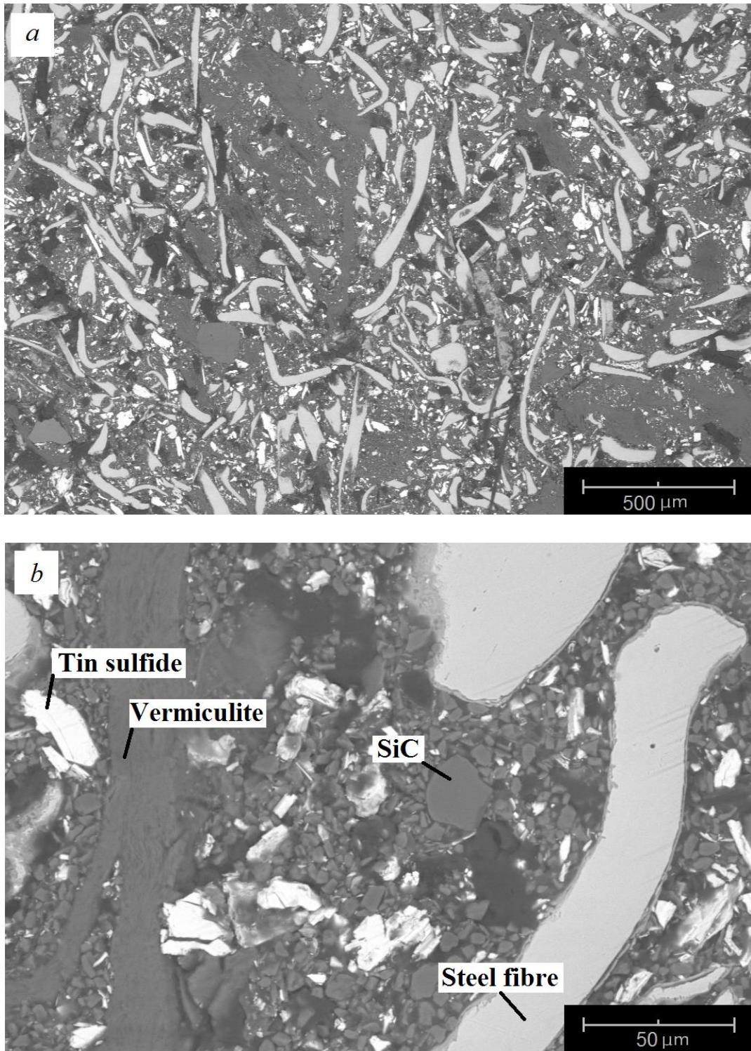
Figure 4.15. BSE images of polished surface PMSQ-HT400 sample at 150x (a) and 1500x (b) magnification.
