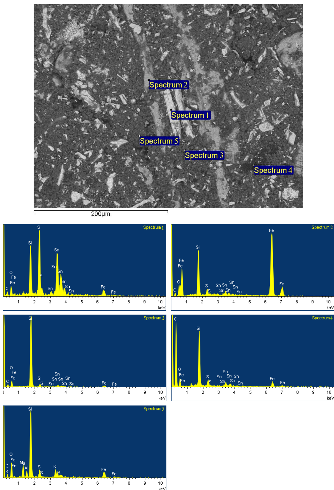
Figure 4.20. EDX point analysis of PMSQ-CL sample at 250 °C. Spectrums show each ingredient in the composite structure; tin sulfide particle, steel fiber, SiC particles, crosslinked polymer and vermiculite particle respectively.
