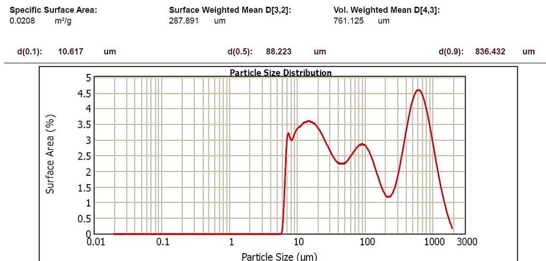
Figure 3.6. Particle size distribution of vermiculite (in ethanol).
