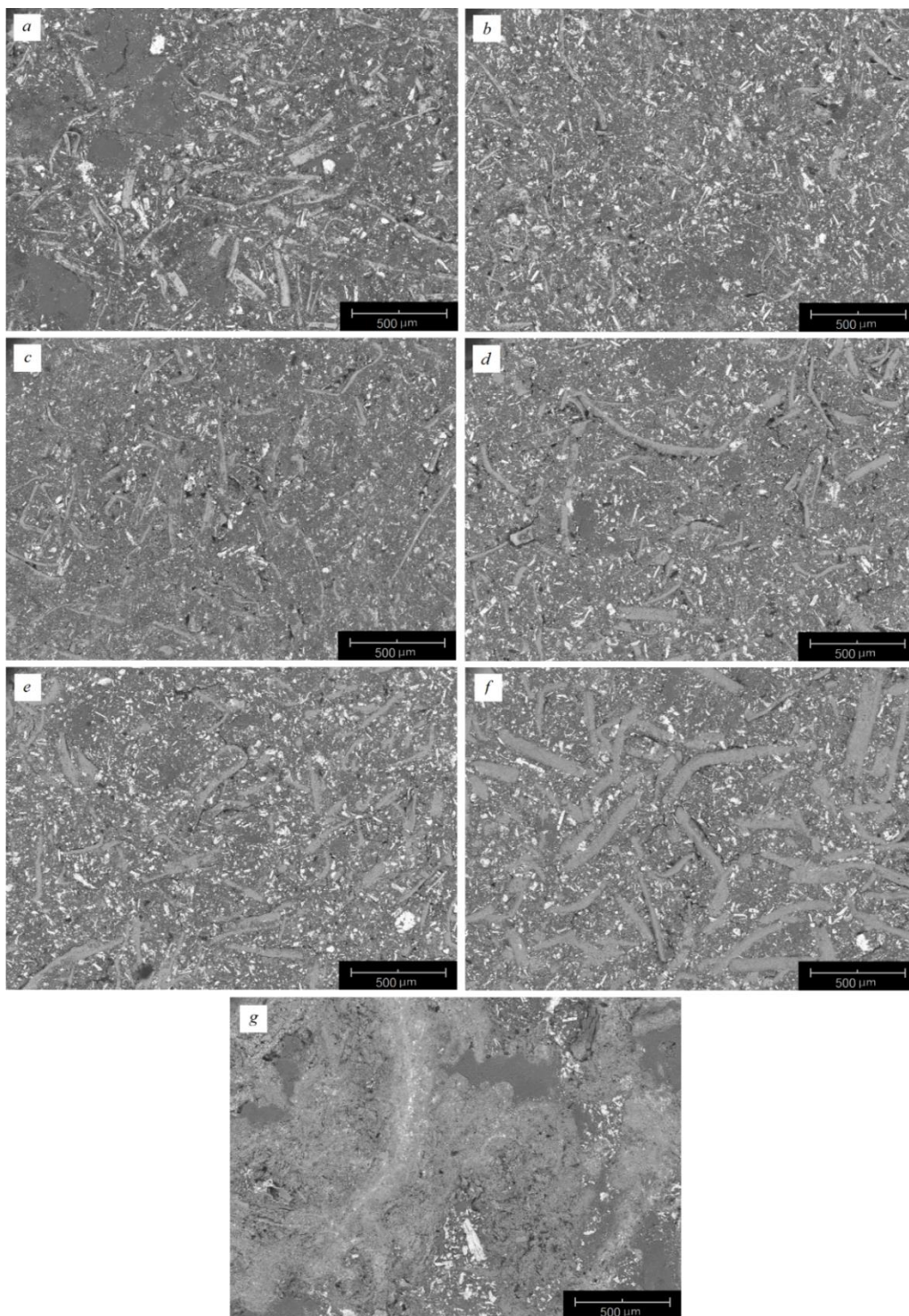
Figure 4.10. BSE images of as pressed surface of PPSQ matrix composite samples in three different conditions at 150x magnification; (a) just warm pressed sample at 150 °C (PPSQ-WP), (b) just crosslinked sample after warm pressing at 300 °C (PPSQ-CL), and heat treated samples at different temperatures after crosslinking (c) PPSQ-HT400, (d) PPSQ -HT500, (e) PPSQ -HT600, (f) PPSQ -HT700, and (g) PPSQ -HT800.
