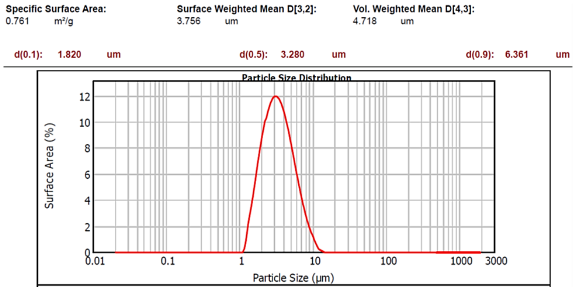
Figure 3.4. Particle size measurement of silicon carbide powder (in water).
