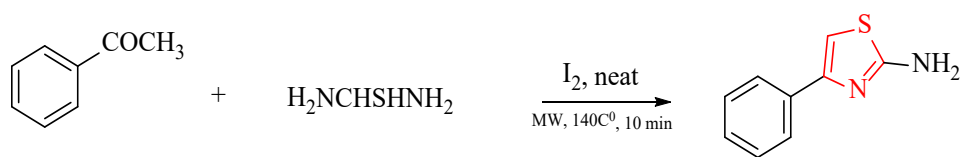
Figure 2.10. Thiazole synthesis using microwave irradiation.
