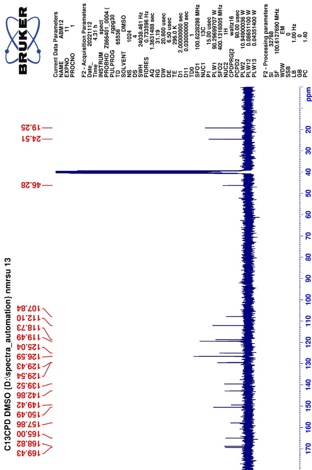
Figure 5.54. ^{13}\text{C} -NMR spectrum of compound 5j
