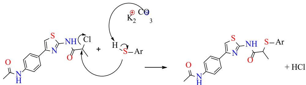
Figure 5.71. Mechanism of method E
