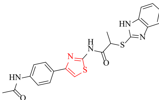
Figure 5.31. Molecular structure of compound 5f
