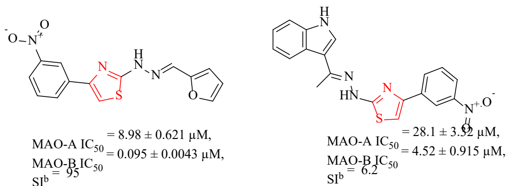
Figure 2.24. (E)-2-[2-(Furan-2-ylmethylene)hydrazinyl]-4-(3-nitrophenyl)thiazole (Left) (E)-2-[2-(1H-Indol-3-yl)ethylidene)hydrazinyl]-4-(3-nitrophenyl)thiazole (Right)
