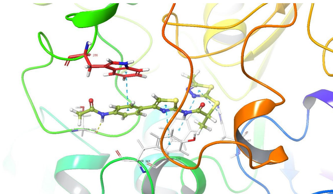
Figure 5.73. 3D interactions of compound 5d at the (4EY7 / PBDID) binding region of AChE
