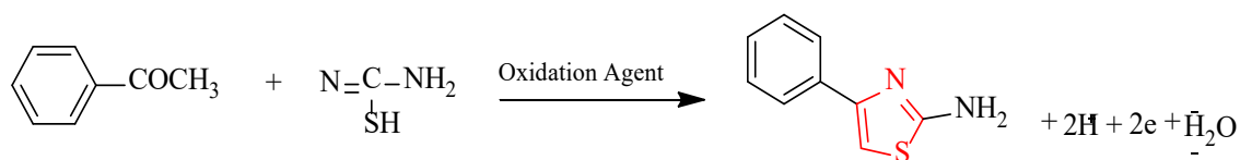
Figure 2.14. Synthesizing of thiazole derivatives utilizing oxidizing agents.
