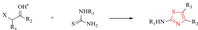
Figure 2.5. Substituted aminothiazole synthesis.
