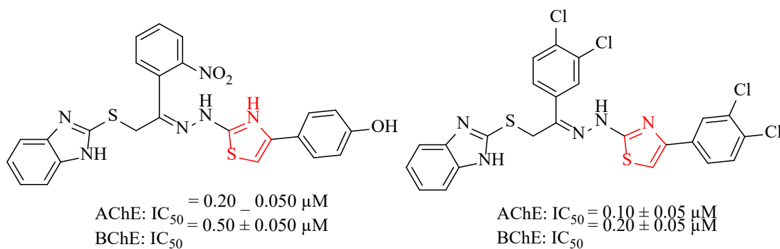
Figure 2.28. ( E )-4-[2-[2-(2-((1 H -Benzimidazol-2-yl)thio)-1-(2-nitrophenyl)ethyldene)hydrazinyl]thiazol-4-yl]phenol (left) ( E )-2-[2-[2-((1 H -benzimidazol-2-yl)thio)-1-(3,4-dichlorophenyl)ethyldene)hydrazinyl]-4-(3,4-dichlorophenyl]thiazole (Right)
