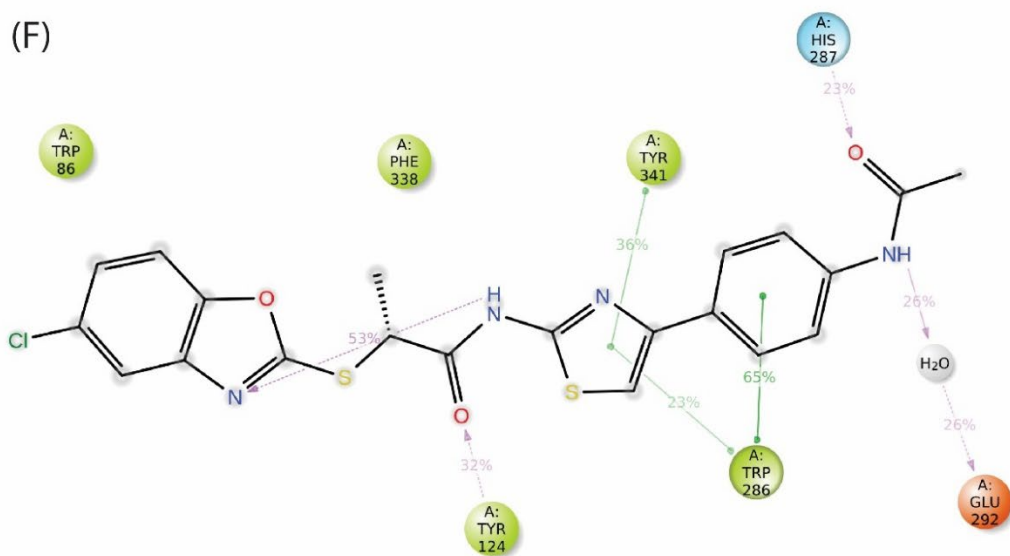
Figure 5.80. MDS Results of 5j ligand with AChE (D) Number of interactions by residue during the simulation., (E) Plot of root mean square fluctuation-residue index (blue: water-mediated H-bond; green: H-bond, pink: ionic interaction, purple: hydrophobic interaction) (F) 2D diagram of the interaction strengths (cutoff=20%)
