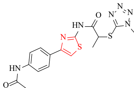
Figure 5.11. Molecular structure of compound 5b
