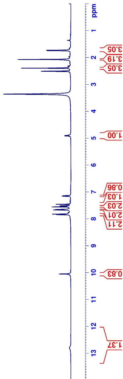
Figure 5.63. ^1\text{H} -NMR spectrum of compound 5I
