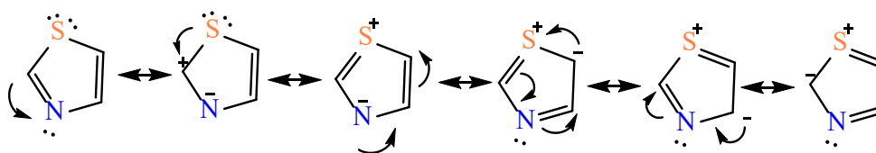
Figure 2.2. Thiazole resonance structures
