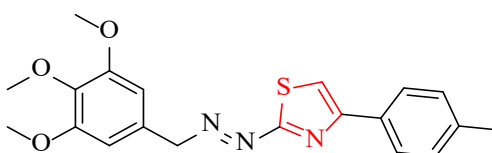
Figure 2.15. N -(4- p -Tolyl-thiazol-2-yl)- N' -(3,4,5-trimethoxy-benzyl)-hydrazine
