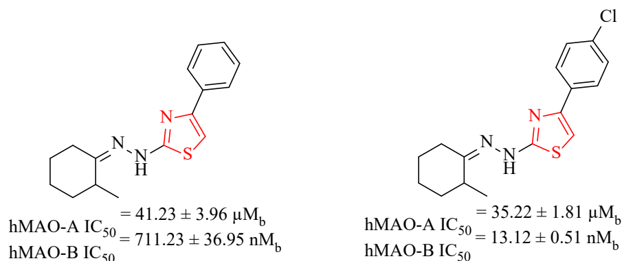
Figure 2.17. (Z)-2-[2-(2-Methylcyclohexylidene)hydrazinyl]-4-phenylthiazole (Left) (Z)-4-(4-Chlorophenyl)-2-[2-(2-methylcyclohexylidene)hydrazinyl]thiazole (Right)
