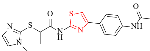
Figure 5.6. Molecular structure of compound 5a
