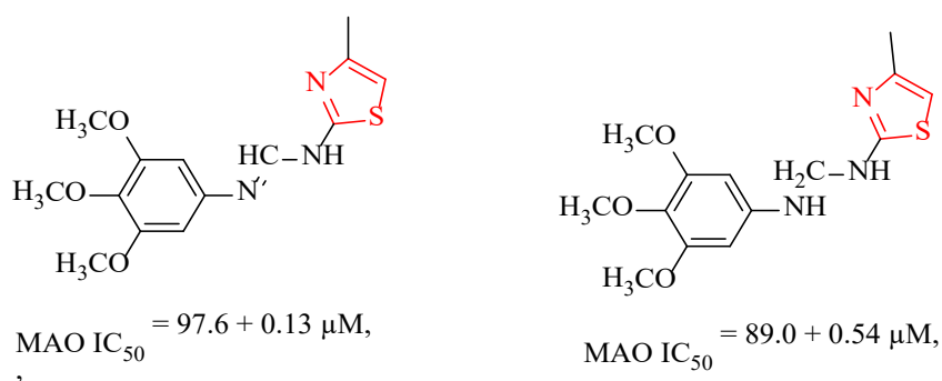
Figure 2.16. ( E )- N -(4-Methylthiazol-2-yl)- N' -(3,4,5-trimethoxyphenyl) formimidamide (Left) N -(4-Methylthiazol-2-yl)- N -(3,4,5-trimethoxyphenyl)methanediimine (Right)
