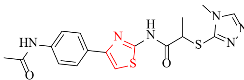
Figure 5.41. Molecular structure of compound 5h
