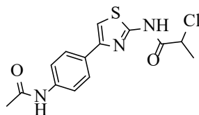
Figure 5.4. Molecular structure of compound (4)
