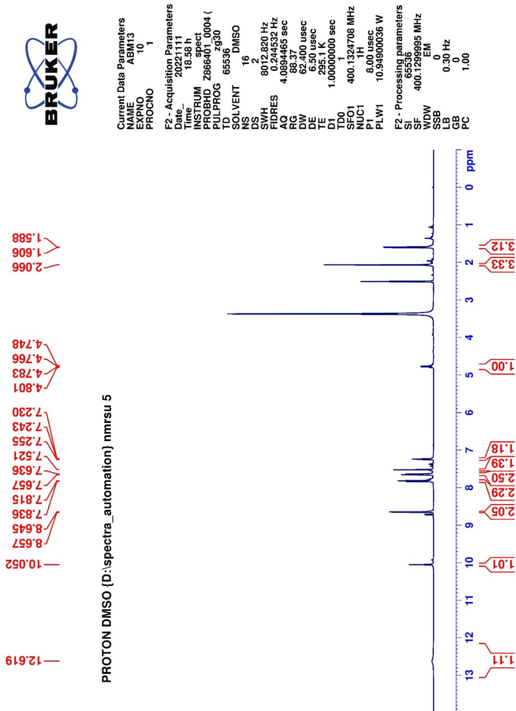
Figure 5.58. 1 H-NMR spectrum of compound 5k
