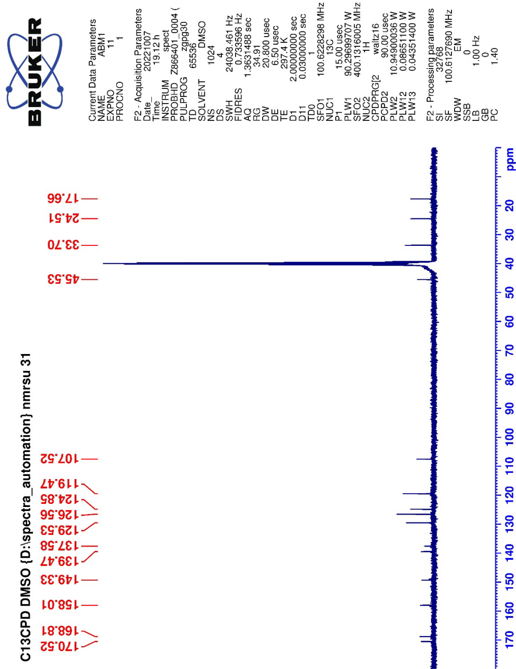
Figure 5.9. 13 C-NMR spectrum of compound 5a
