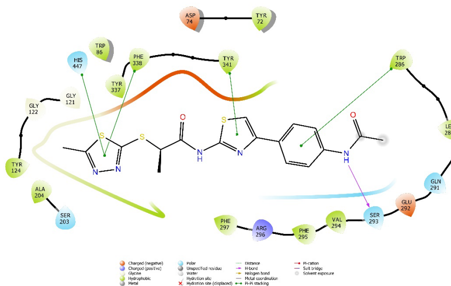
Figure 5.74. 2D interactions of compound 5d at the (4EY7 / PBDID) binding region of AChE
