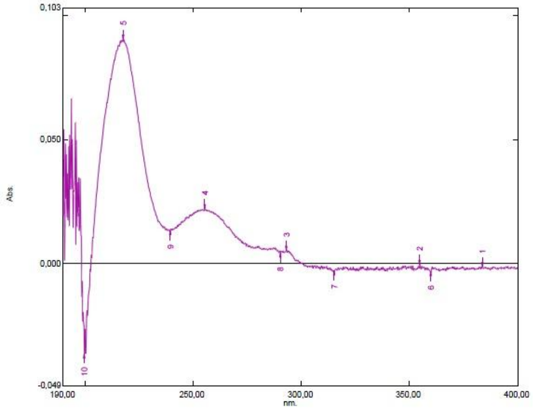
Şekil 6. 1.01 \times 10^{-6} M ARP spektrumu (4: 255.40 nm, 5: 217.80 nm)
