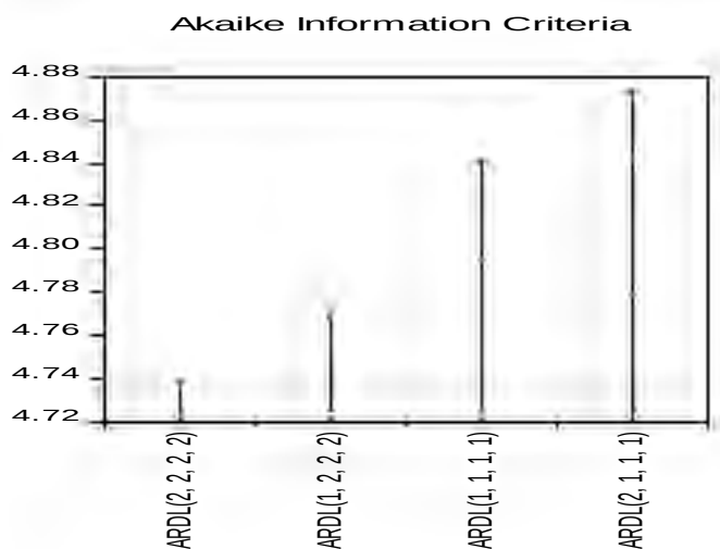
Figure: 2.3: Model Selection summary using AIC
