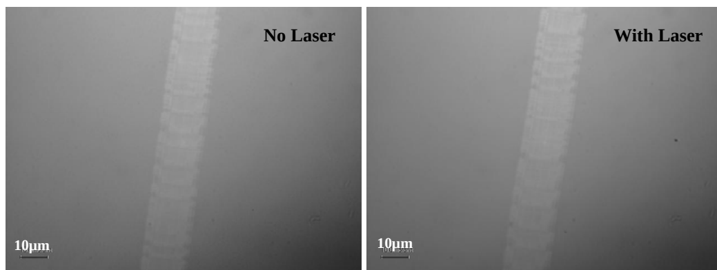
Figure 9.18. Image of part of the scratch done with a 20mN (2g) thrust force. (No visual difference seen under the optical microscope between a scratch done with and without laser heating. The image was taken at a 1000x magnification. The width of the scratches are approximately 17µm).
