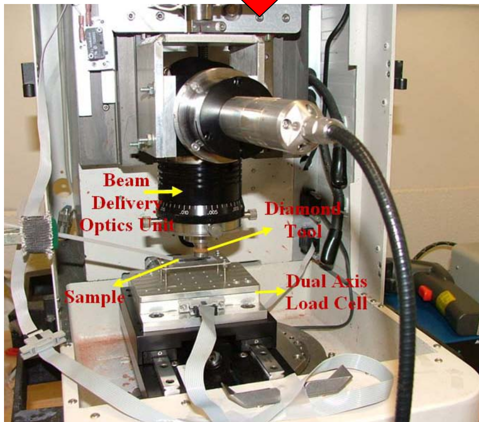
Figure 10.4. IPG Laser system coupled with a laser beam delivery optics unit.
