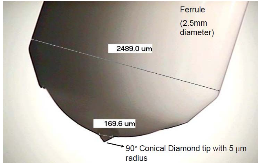
Figure 7.3. 90°conical single crystal diamond tip with 5 μm radius spherical end attached on the end of the ferrule using epoxy.
