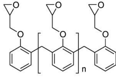
Phenol Novolac Epoxy
