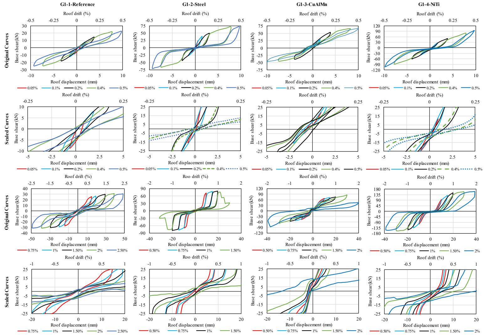
Figure 5.17. Comparison of hysteresis curves in re-centering property
