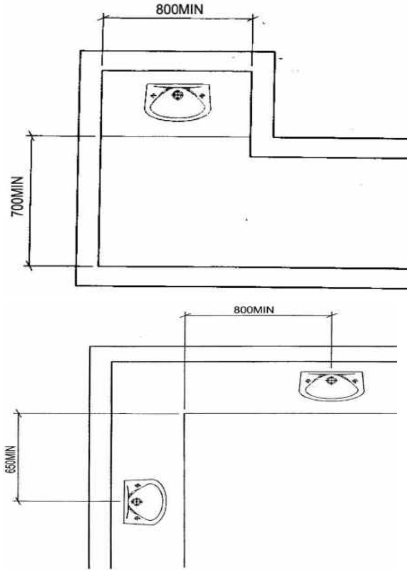
Görsel 2.9. Lavabo ile çevre ilişkisi (Restroom Association. 2014. A Guide to Better Preschool Toilet Design, Maintenance and Education. s.55-56.)
