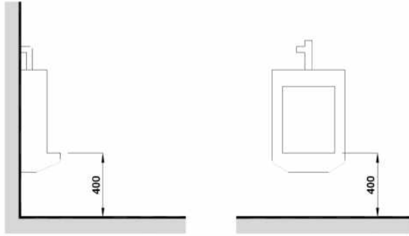
Görsel 2.10. Pisuvar ölçüleri (Restroom Association. 2014. A Guide to Better Preschool Toilet Design, Maintenance and Education. s.41.)
