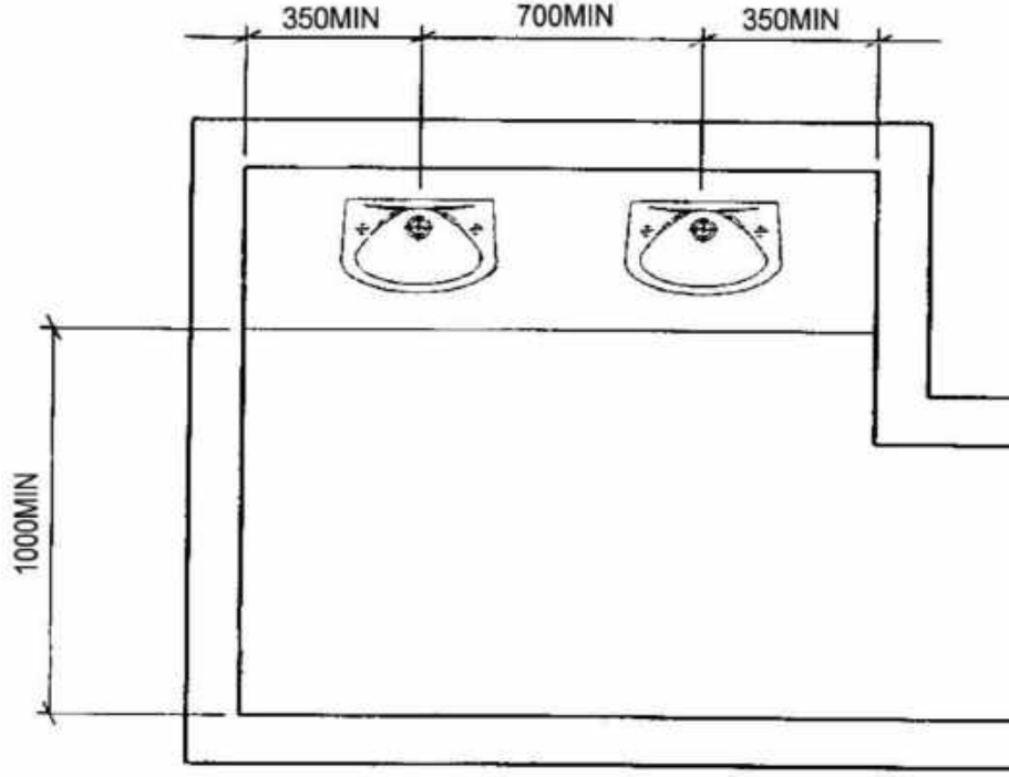
Görsel 2.3. El yıkama bölümü (Restroom Association. 2014. A Guide to Better Preschool Toilet Design, Maintenance and Education. s.55-56.)
