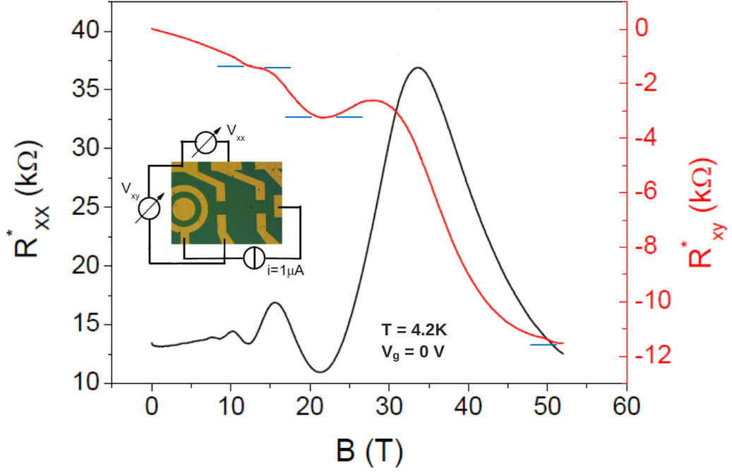
Figure 6.8. Longitudinal ( R_{xx} ) and Hall ( R_{xy} ) resistance measured as a function of magnetic field of up to 53T. The horizontal lines correspond to h/e^2\nu values, where the quantized plateaus are expected.
