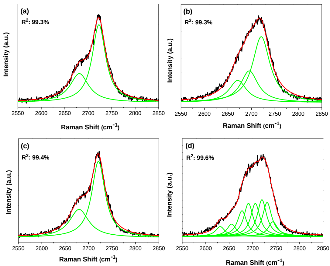
Figure 3.15. The enlarged 2D-band regions (of Fig. 1) with Lorentzian curve fittings of (a) , (b) expandable graphite, (c) expanded graphite (EG), and (d) exfoliated sample (EG-IPA-90min-TS). The black, green and the red curves represent the spectra, fit peaks and the cumulative fit peak, respectively.
