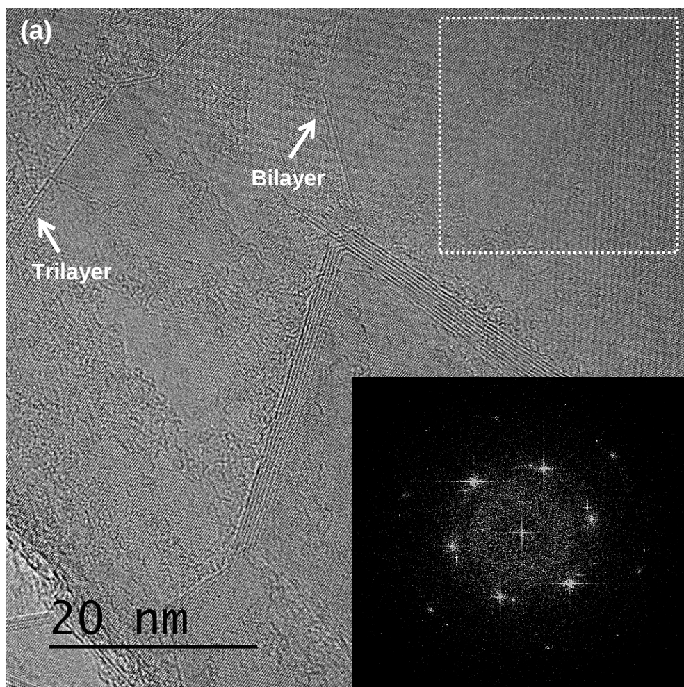
Figure 3.26. HRTEM images of SEFG-IPA-90m sample annealed at 2600°C in Ar atmosphere for 4 h revealing bi-layer and few-layer (<5 layers) graphene sheets (a) , (b) . Inset in (a) show the corresponding FFT image of the region indicated by the dashed rectangle and inset in (b) is the corresponding FFT image of the micrograph shown in (b).
