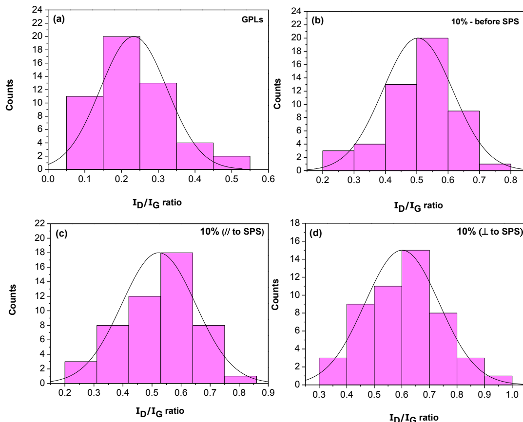
Figure 4.11. Statistical histogram of the D-band intensity to G-band intensity ratios ( I_D/I_G ) derived from 50 Raman spectra. (a) Initial GPLs, (b) 10 vol.% GPLs/ Al_2O_3 powder (before SPS), (c) 10 vol.% GPLs/ Al_2O_3 nanocomposite in through-thickness direction, and (d) 10 vol.% GPLs/ Al_2O_3 nanocomposite in in-plane direction. The distribution curves indicate the mean of the data.
