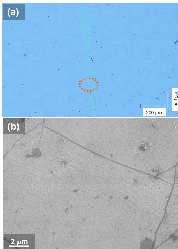
Figure 5.16. (a) Optical image and (b) FEG-SEM micrograph of the graphene film grown on B2 Cu foil, which was pre-cleaned by nitric acid for 60 s (using 200 sccm Ar/100 sccm \text{H}_2 during ramping, 100 sccm \text{H}_2 /17 sccm \text{CH}_4 during graphene growth for 5 min, and 0.3 torr and 0.2 torr pressure during ramping and annealing steps, respectively) and transferred onto a \text{SiO}_2 (300 nm)/Si substrate.
