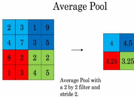
Figure 4.15. Average pooling function
