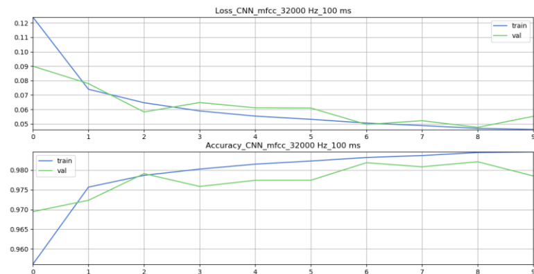
Figure 4.61. Accuracy and loss during model's training
