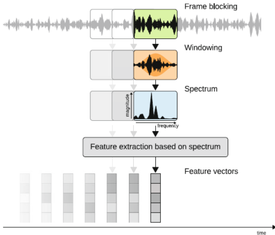
Figure 4.7. The processing pipeline of feature extraction techniques
