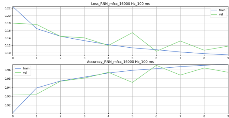
Figure 4.29. Accuracy and loss during training
