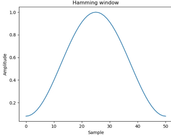
Figure 4.8. Hamming window
