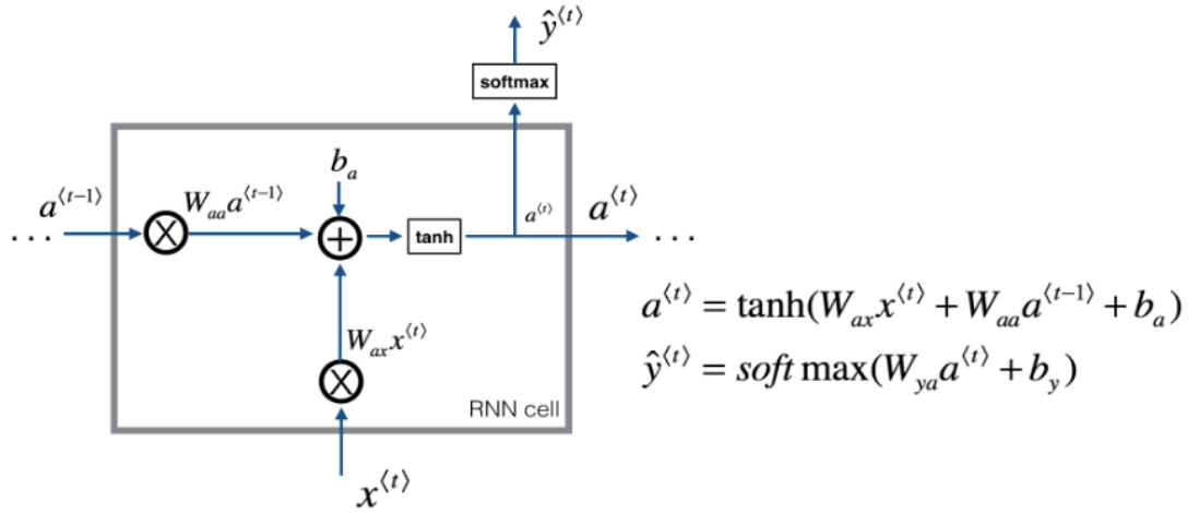
Figure 4.18. Basic cell in recurrent neural network
