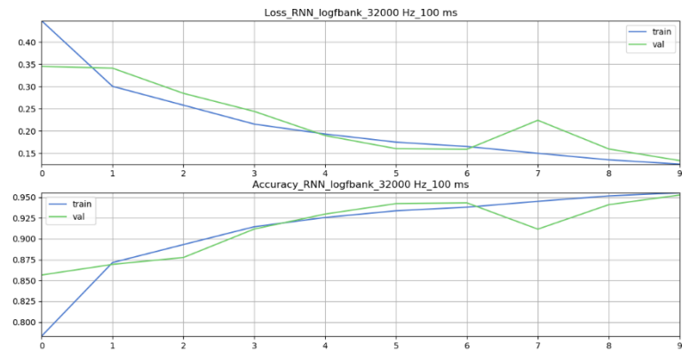
Figure 4.41. Accuracy and loss during training
