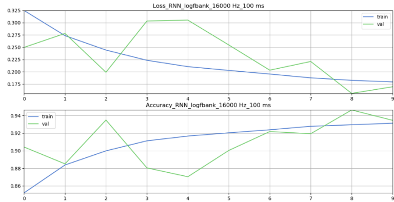
Figure 4.33. Accuracy and loss during training
