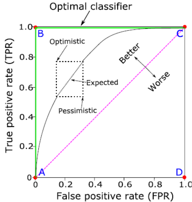
Figure 4.26. Receiver operating curve (ROC)
