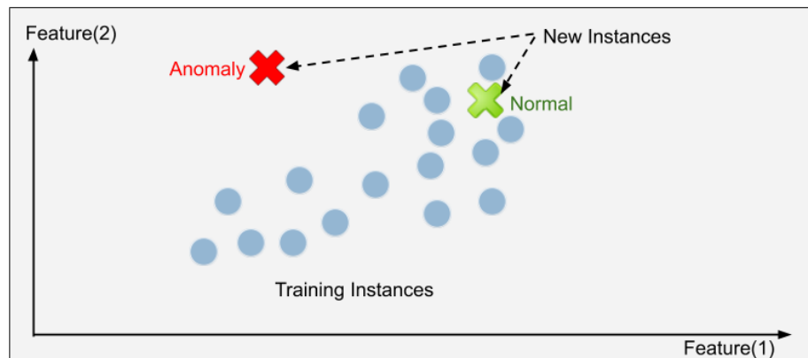
Figure 3.4. Anomaly detection
