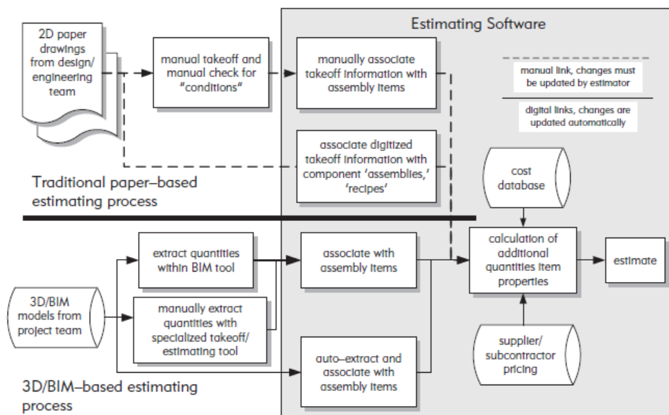
Figure 3.16. Traditional paper based and 3D BIM based estimation process (Eastman et al., 2011)
