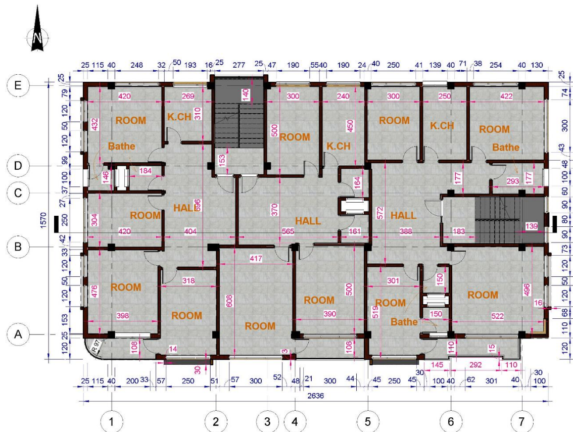
Figure 5.4. Typical floors plan of 4 story building
