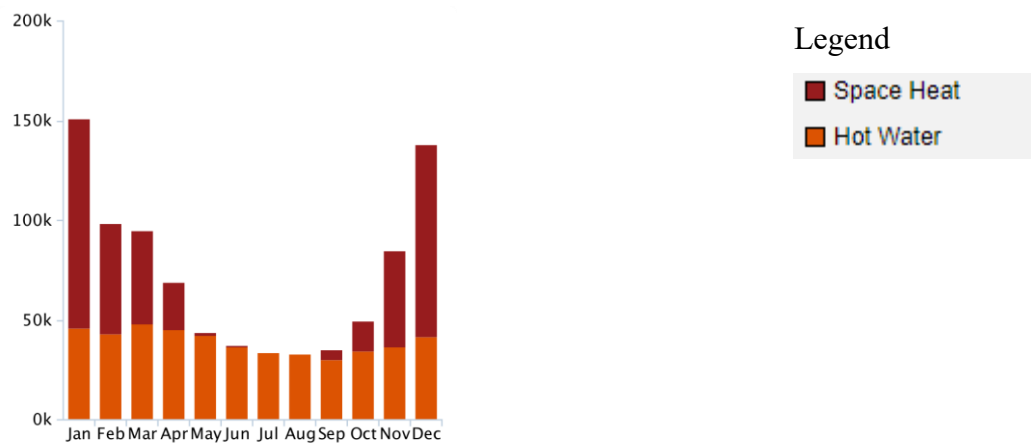
Figure 6.18. Monthly fuel (Natural gas) use for alternative design (MJ)
