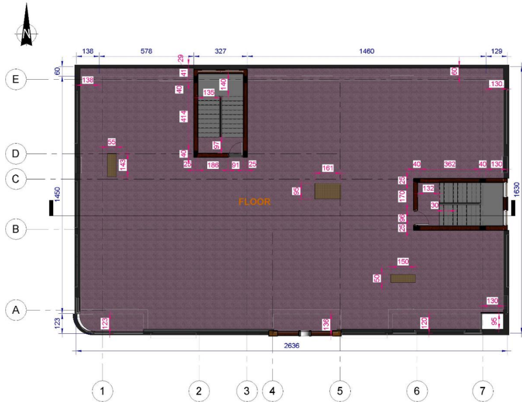
Figure 5.5. Roof plan of 4 story building
