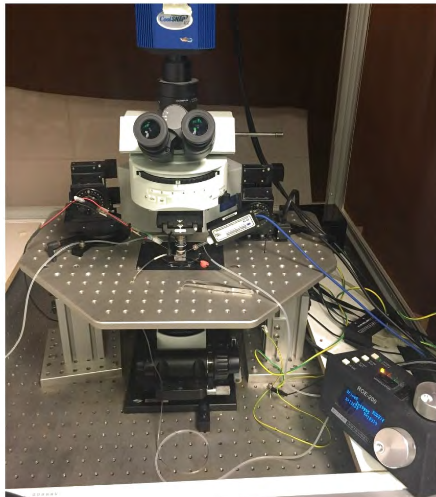
Figure 3.3. Electrophysiology rig
