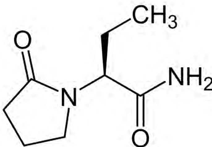
Figure 2.4. Chemical structure of LEV ((-)-S)- \alpha -ethyl-2-oxo-1-pyrrolidine acetamide, C_8H_{14}N_2O_2 )
