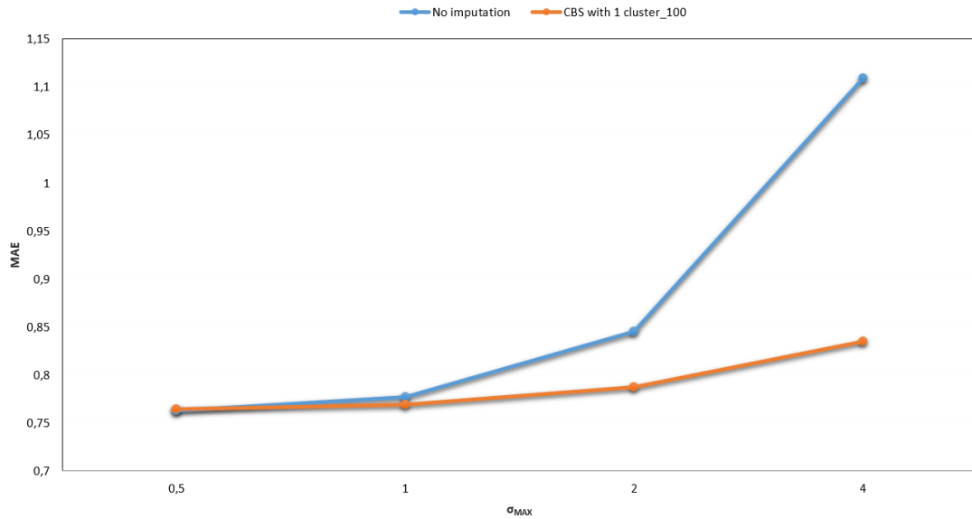
Figure 5.8. MAE results on user-based PPCF by varying \sigma_{max} value comparing CBS imputation with no imputation. Cluster count and filling percentage are adjusted as 1 and 100 respectively for CBS.
