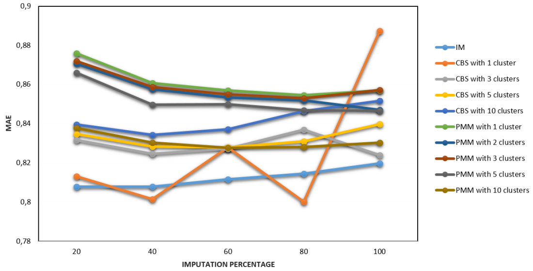
Figure 5.3. Comparison of MAE results for imputed clustering-based PPCF with 2 clusters by varying imputation percentage
