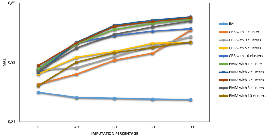
Figure 5.2. Comparison of MAE results for imputed SVD-based PPCF by varying imputation percentage
