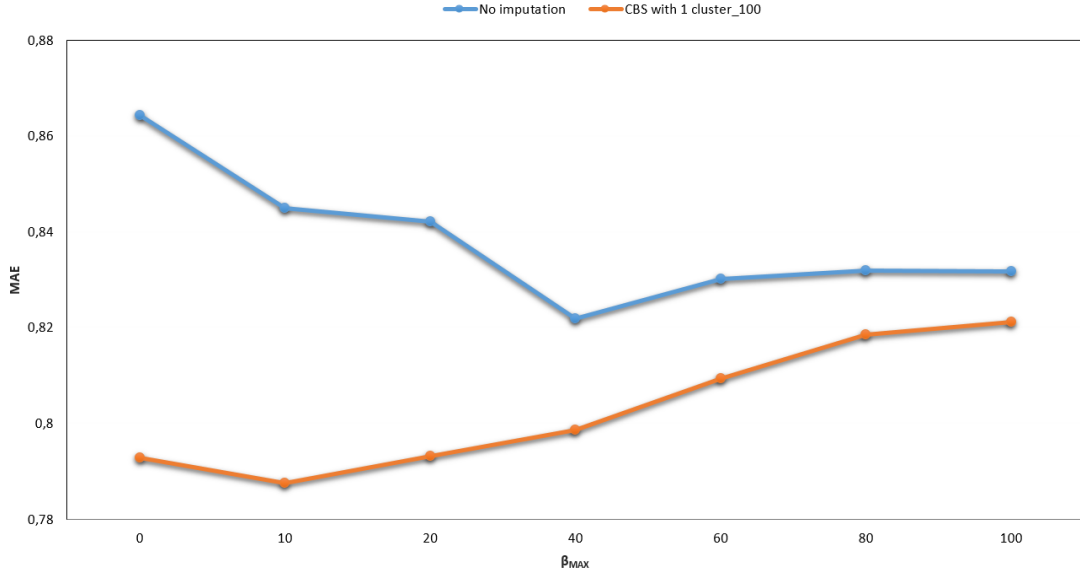
Figure 5.7. MAE results on user-based PPCF by varying \beta_{max} value comparing CBS imputation with no imputation. Cluster count and filling percentage are adjusted as 1 and 100 respectively for CBS.
