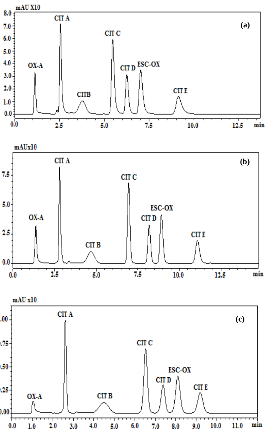
Figure 5.12. Chromatogram of ESC-OX and its Impurities by Using; (a) Nucleosil ® 100 C 18 (3 \mu m, 10 \times 0.46 cm), (b) Synergi Hydro-RP ® (4 \mu m, 15 \times 0.46 cm), (c) Fluophase RP ® (3 \mu m, 10 cm \times 4.6 mm).
