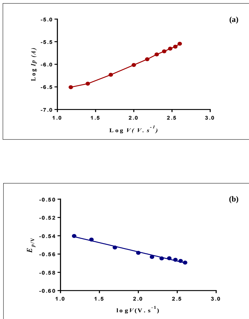
Figure 5.40. (a) The Linear Dependence of the Logarithm of the Peak Current ( \text{Log } I_{pc} ) of ESC-OX on the Logarithm of the Potential Scan Rate ( \text{Log } v ); (b) the Reliance of the Peak Potential ( E_p ) of ESC-OX on the Logarithm of Potential Scan Rate ( \text{Log } v ).
