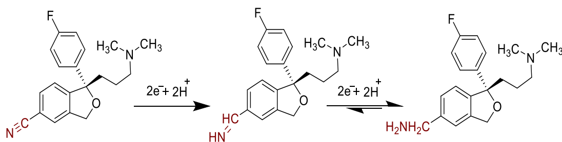
Scheme 5.1. Proposed Reduction Mechanism of ESC-OX.
