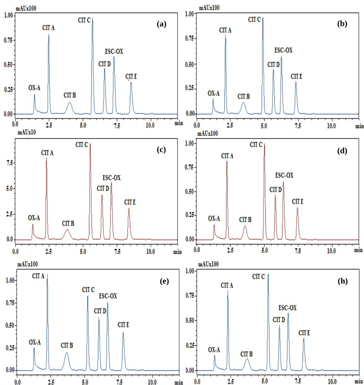
Figure 5.29. The Chromatogram of Robustness Study by Using (a) Flow Rate 1.1 min mL -1 , (b) Flow Rate 1.3 min mL -1 , (c) Temperature 35°C, (d) Temperature 45°C, (e) Wavelength 205 nm (f) Wavelength 215 nm.
