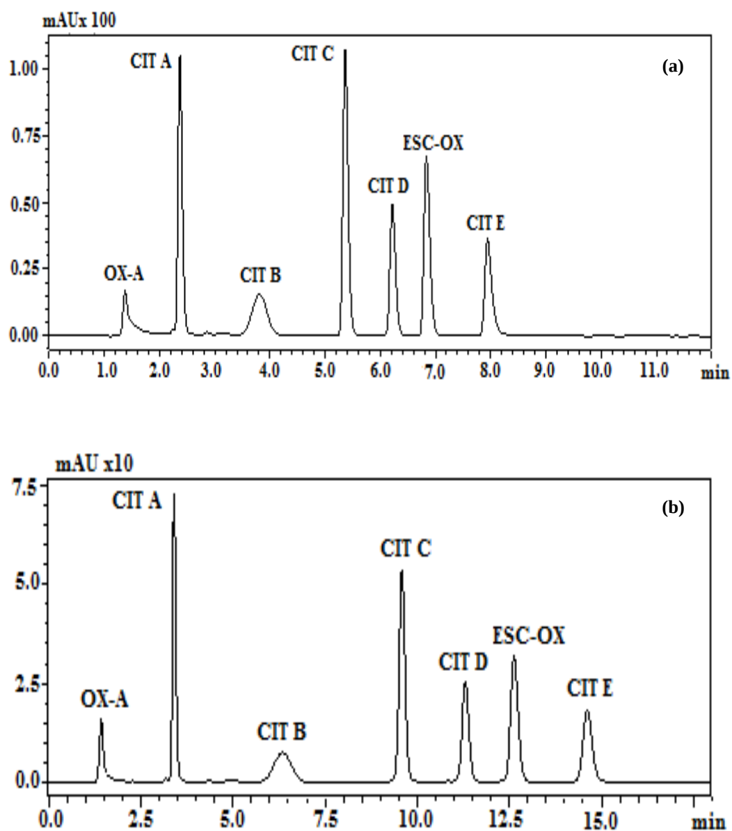
Figure 5.16. Chromatogram of Standard Solution of ESC-OX and its Impurities by using (a) Kinetex ® Phenyl-Hexyl (2.6 \mu m, 150 \times 4.6 mm) Core-Shell Column. (b) Luna ® Phenyl-Hexyl (2.6 \mu m, 150 \times 4.6 mm) Fully Porous Column.
