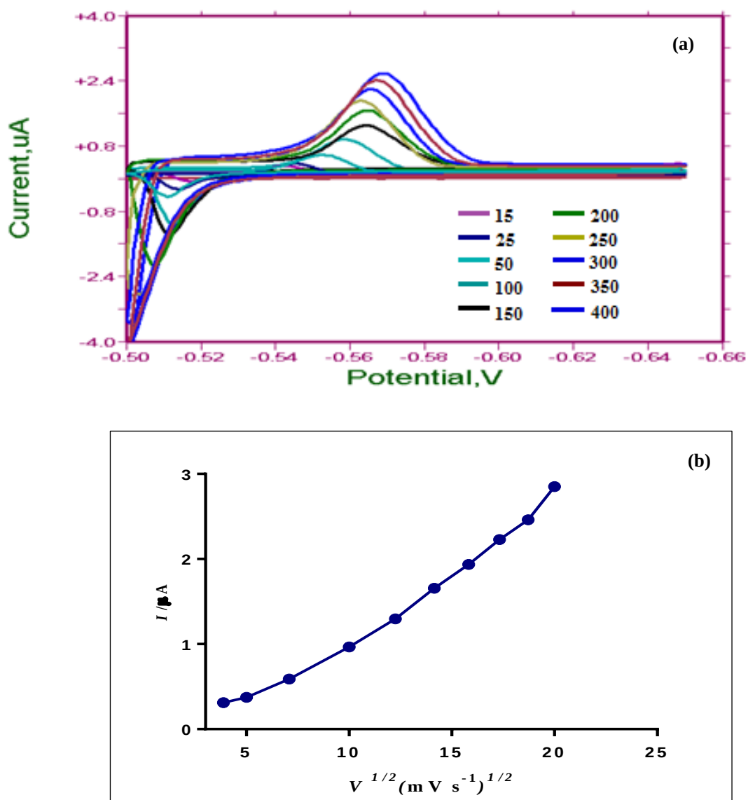
Figure 5.39. (a) Cyclic Voltammograms of ESC-OX ( 41.44 \mu\text{g mL}^{-1} ) Recorded in the BR Buffer (pH 6.5), KCl (0.3 M) and 5% MeOH on HMDE at Various Scan rate, (b) the Linear Dependence of the ( I_{pc} ) of ESC-OX on the Square Root of the Potential Scan Rate ( v^{1/2} ).
