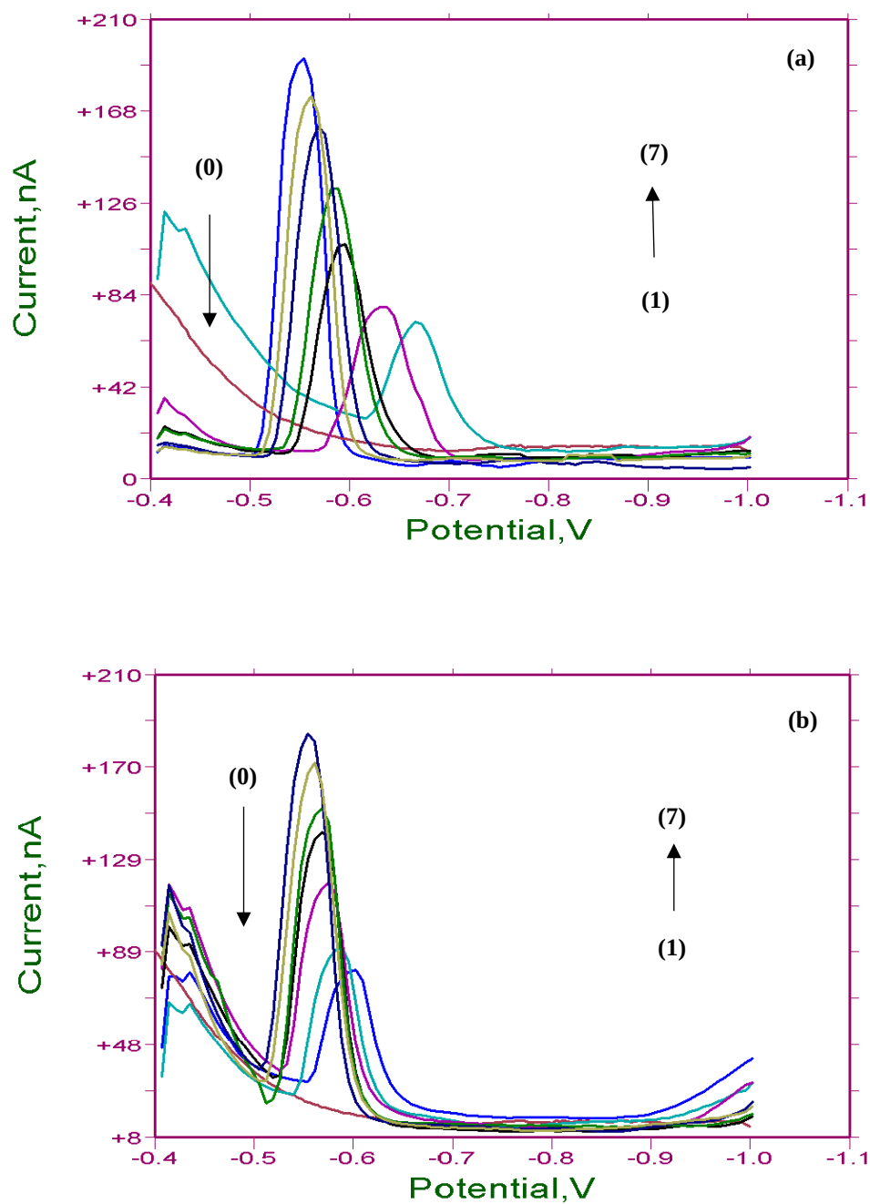
Figure 5.43. DP Voltammograms of ESC-OX Recorded in BR buffer, pH 3.5, 3M KCl, 5% MeOH. The Concentrations of the ESC-OX Increase in the Following Manner: (0) Blank, (1) 4.14, (2) 8.28, (3) 12.43, (4) 16.56, (5) 20.72, (6) 24.86, (7) 29.00 \mu\text{g mL}^{-1} . (b) DP voltammograms of ESC-OX recorded in spiked human urine.
