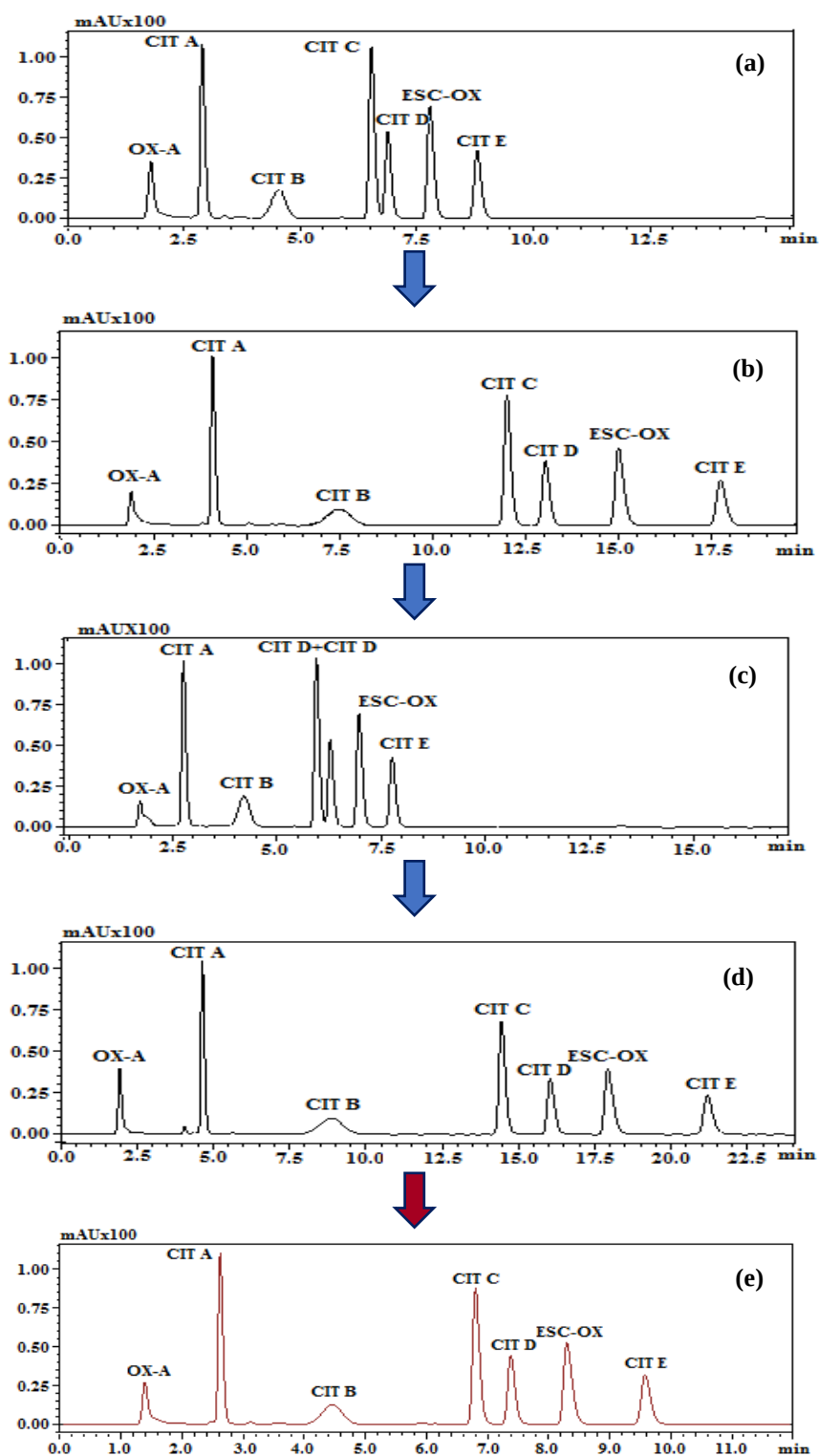
Figure 5.11. The Chromatograms Related to the Method Development by Using Kinetex ® PFP Core-Shell Column (a) Buffer: ACN: H 2 O (50:30:20) v/v/v/v, (b) Buffer: ACN: H 2 O (50:25:25) v/v/v/v, (c) Buffer: ACN: MeOH: H 2 O (50:30:5:15) v/v/v/v, (d) Buffer: ACN: MeOH: H 2 O (50: 20:10:20) v/v/v/v, (e) Buffer: ACN: MeOH: H 2 O (50:25:5:20) v/v/v/v).
