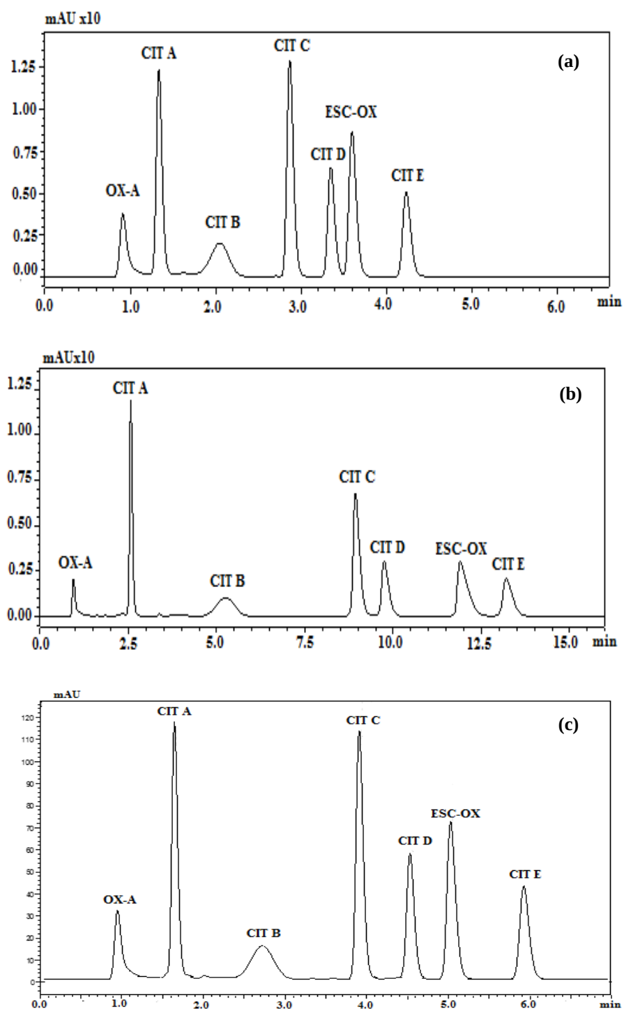
Figure 5.13. Chromatogram of ESC-OX and its Impurities by Using; (a) Ascentis® Express C 18 (2.7 \mu m, 10 cm \times 4.6mm), (b) Ascentis® Express F5 (2.7 \mu m, 10 cm \times 4.6mm), (c) Ascentis® Express Phenyl-hexyl (2.7 \mu m, 10 cm \times 4.6mm).
