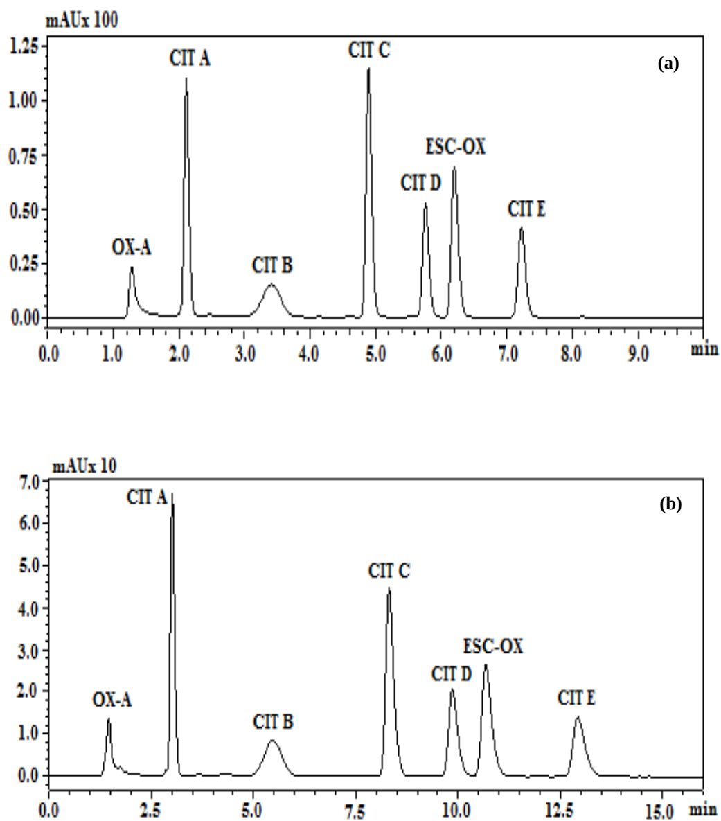
Figure 5.14. Chromatogram of Standard Solution of ESC-OX and its Impurities by Using (a) Kinetex ® C 18 (2.6 \mu m, 150 \times 4.6 mm) Core-Shell Column, (b) Inertsil ® C 18 (3 \mu m, 150 \times 4.6 mm) Fully Porous Column.
