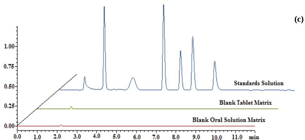
Figure 5.26. Chromatograms Comparison for Blank with ESC-OX and it impurities (a) C_{18} Core-Shell Column, (b) PFP Core-Shell Column, (c) Phenyl-Hexyl Core-Shell Column.
