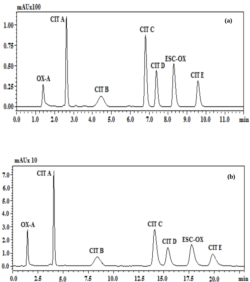
Figure 5.15. Chromatogram of Standard Solution of ESC-OX and its Impurities by (a) Kinetex ® PFP (2.6 \mu m, 150 \times 4.6 mm) Core-Shell Column, (b) Luna ® PFP (2.6 \mu m, 150 \times 4.6 mm) Fully Porous Column.
