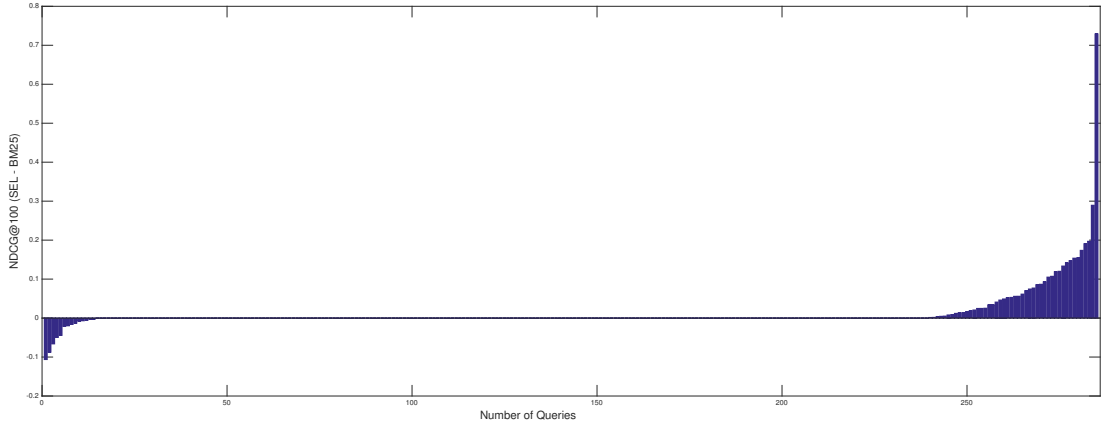
Figure 6.1. ClueWeb{09A|12B} (Anchor): Selective term-weighting SEL is compared with the BM25 term-weighting, which is applied uniformly to all 285 queries, in terms of their \text{NDCG@100} differences. Right side of the figure shows the queries that SEL performed better than BM25 .
