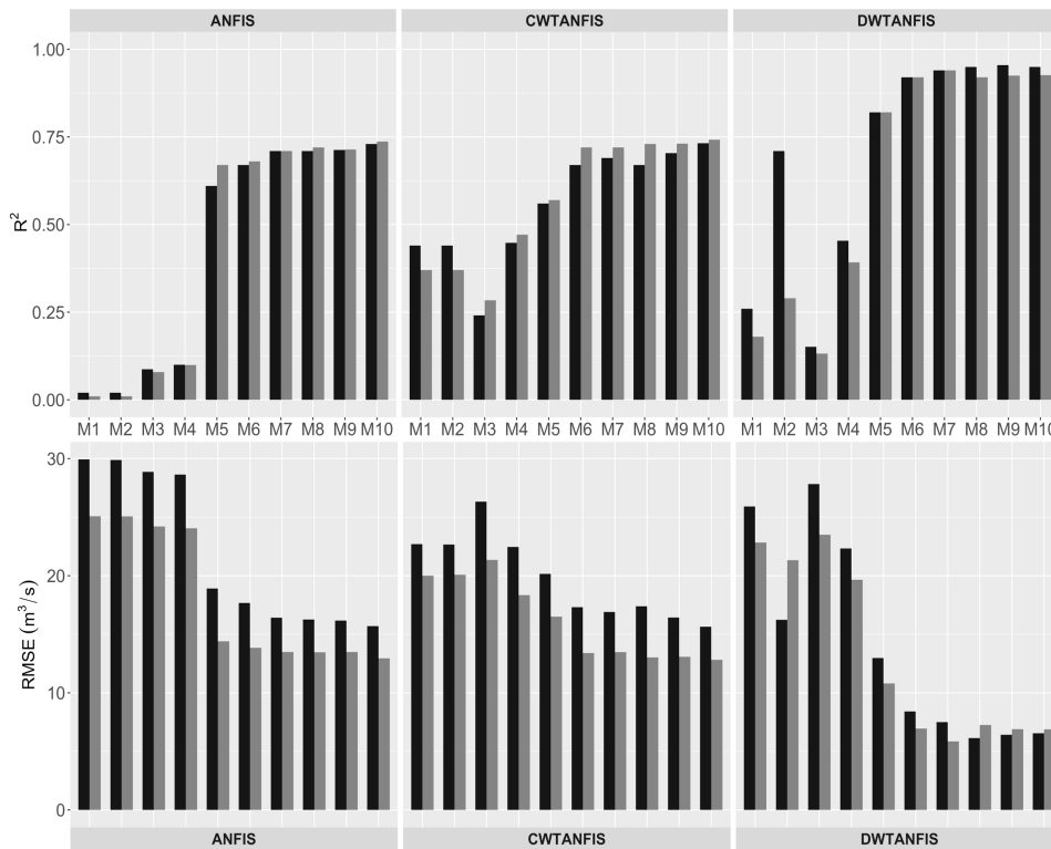
Figure 4.7. The R^2 and RMSE values of the three schematic layouts (ANFIS, CWTANFIS, and DWTANFIS)
