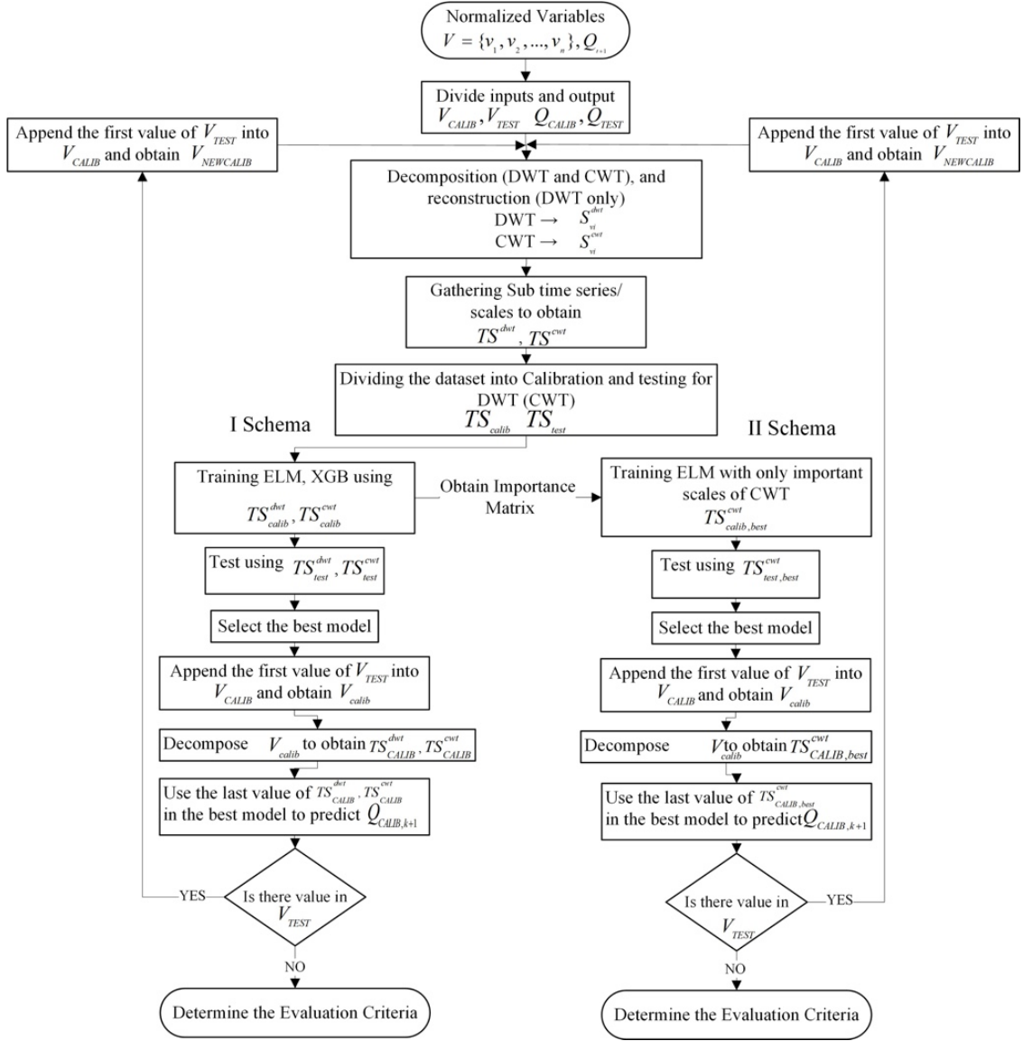
Figure 5.5. The framework of the forecast experiment
