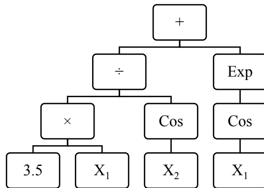
Figure 4.11. GP tree structure of the expression 3.5X_1 \div \text{Cos}(X_2) + \text{exp}(\text{Cos}(X_1))
