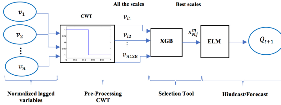
Figure 5.1. Framework of the proposed model schema
