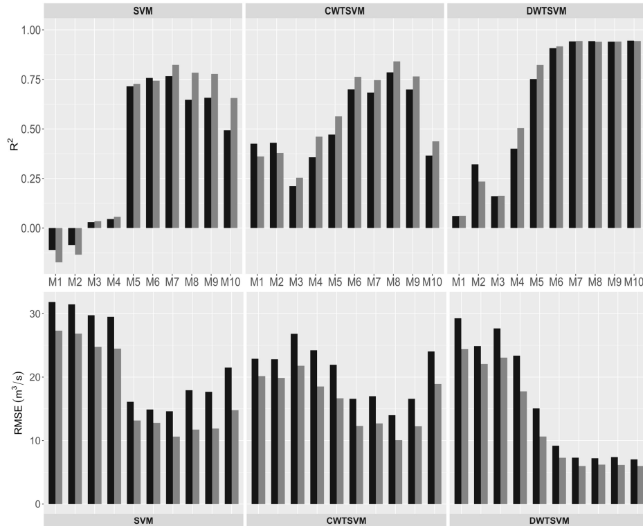
Figure 4.8. The R^2 and RMSE values of the three schematic layouts (SVR, CWT SVM, and DWT SVM)
