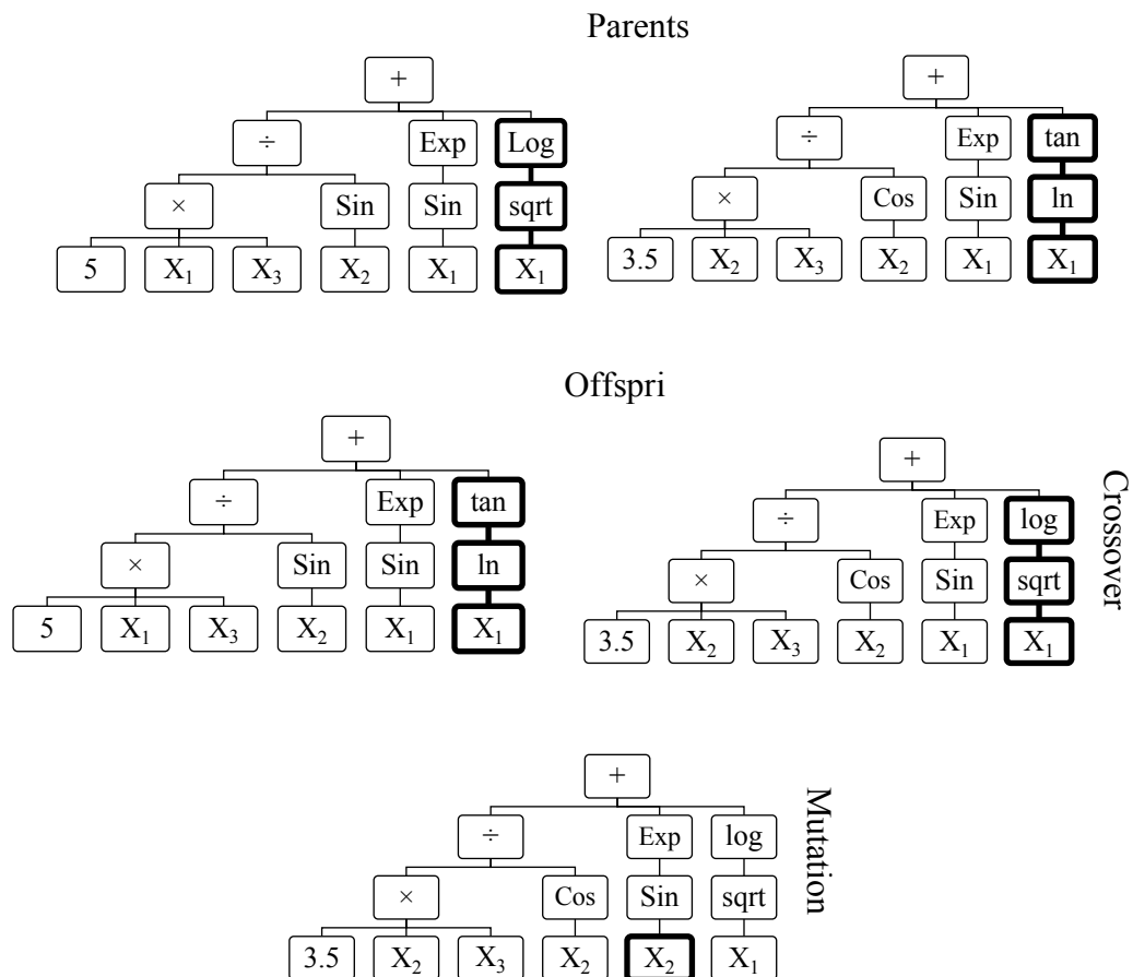
Figure 4.12. An example of the crossover and mutation operations
