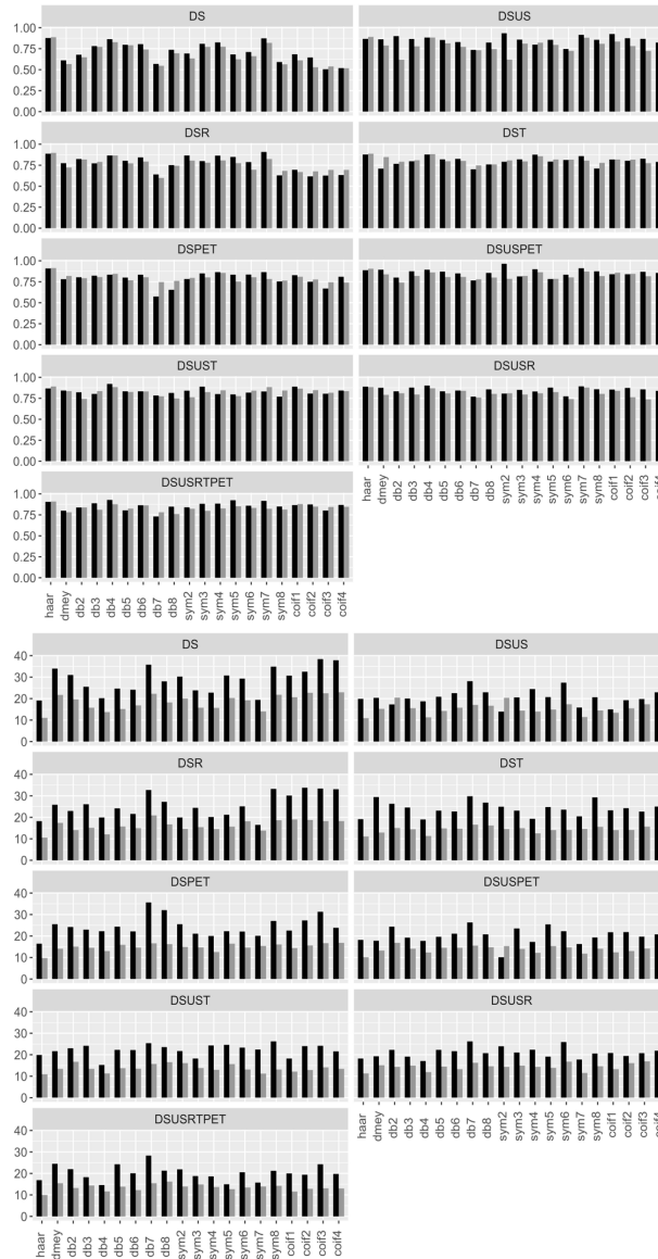
Figure 4.19. The performance of the Best-Scale layout model of the ANN. Top figures ( R^2 ), Bottom figures (RMSE), Black colour: Training subset, Grey Colour: Validation subset
