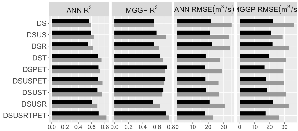
Figure 4.18. The performance of the stand-alone layout models. Black colour: Training subset, Grey Colour: Validation subset
