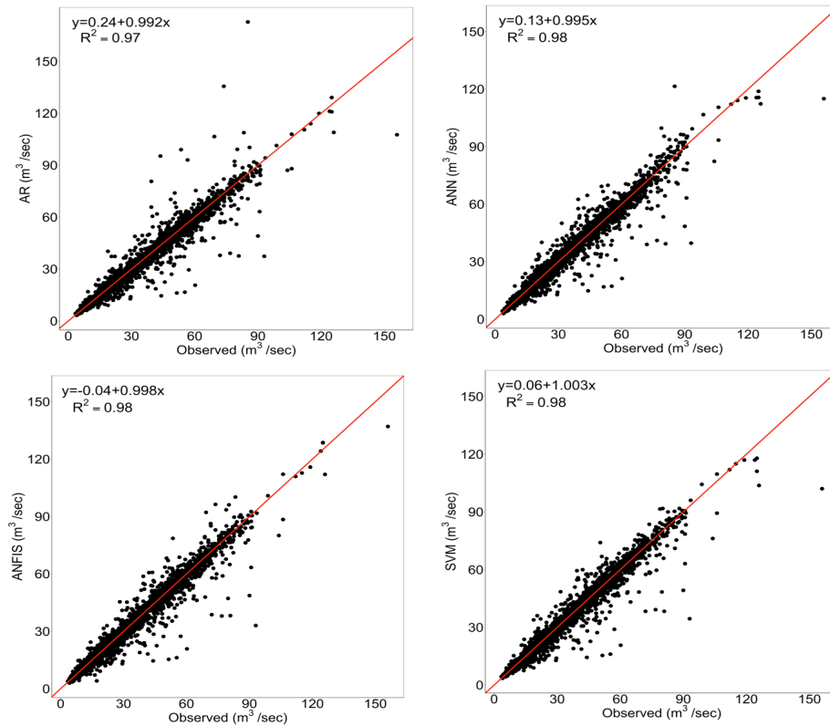
Figure 3.9. Daily streamflow observed vs estimated of the 1822 station. Red lines represent the best fit line
