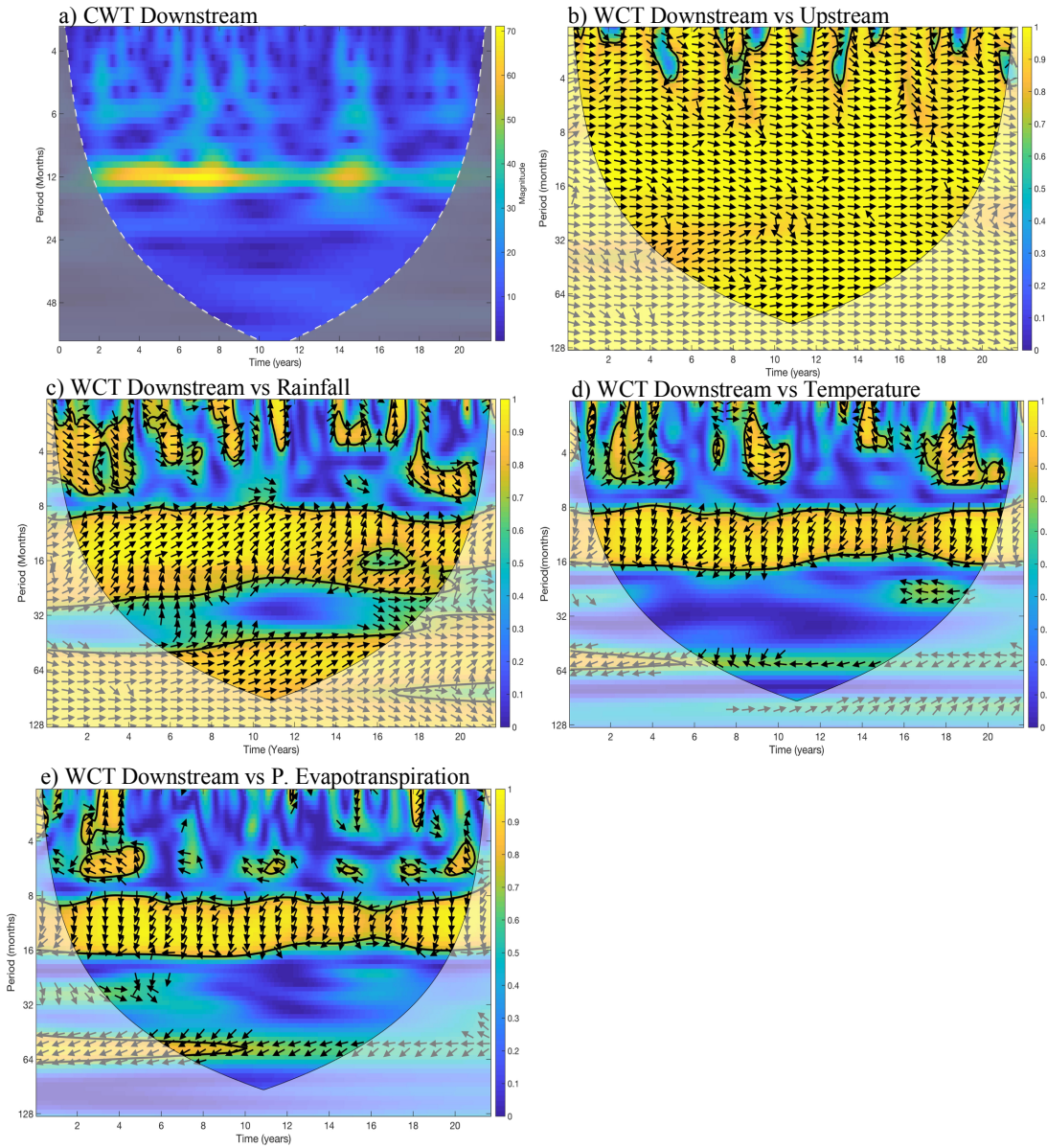
Figure 4.17. a) The CWT scalogram of the downstream, b, c, d, and e) The wavelet coherence scalogram of the downstream with the Upstream, Rainfall, Temperature, and Potential evapotranspiration. The surrounded areas with solid black lines are significant regions in 5% significance level. The arrows represent the phase difference between the two time series. The direction of the Arrows has the meaning; right pointing: in-phase, left pointing: Anti-phase, down pointing: x leads y by 90^\circ (or y lags x by 270^\circ ), up pointing: y leading x by 90^\circ (or x lags y 270^\circ )
