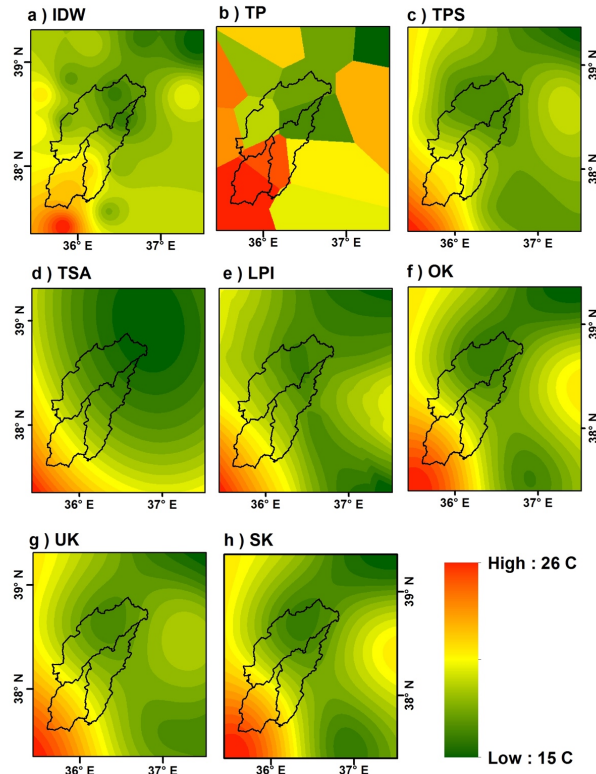
Figure 1.3. Examples of interpolated maps of monthly average temperature (in C°) for each of the 8 interpolation methods. The month chosen as an example is June 1989
