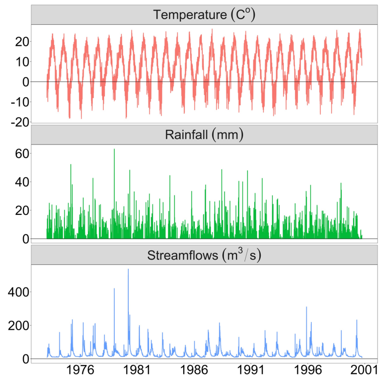
Figure 4.3. Time series of the temperature, rainfall, and streamflow
