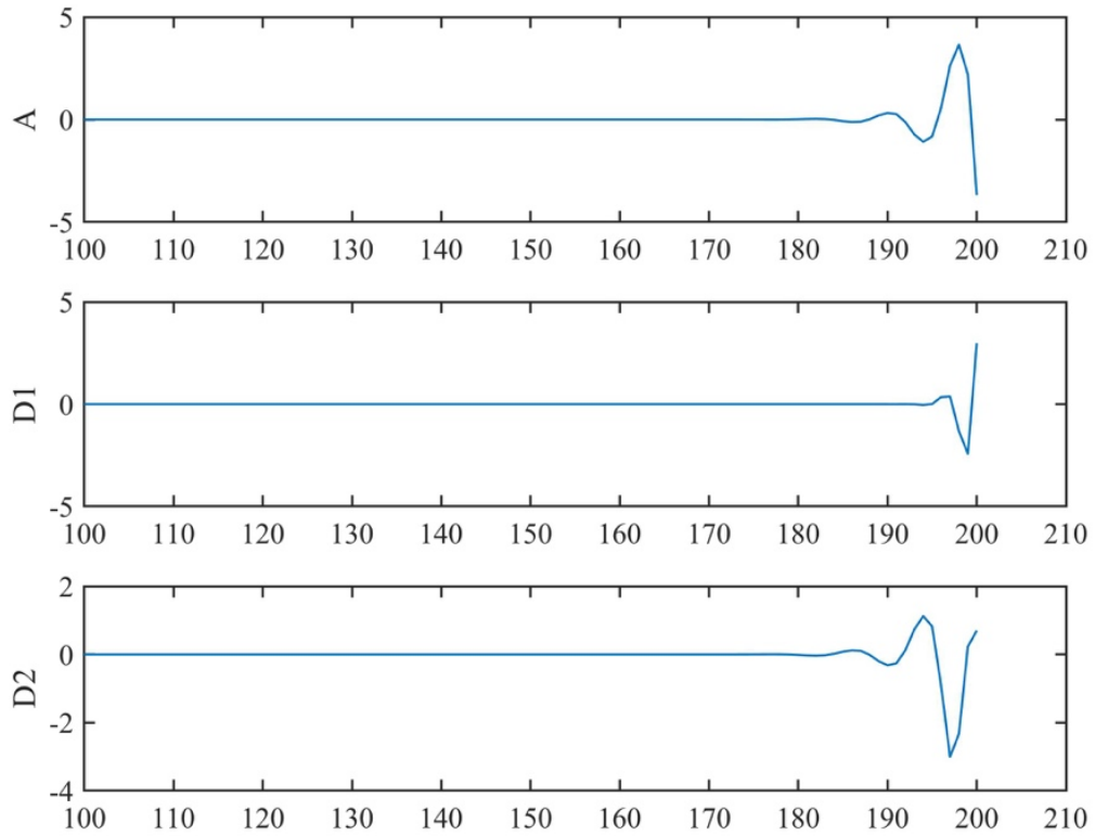
Figure 5.8. The difference between the first 200 steps of sub time series of the downstream flow using DWT with level 2 for 200 and 256 months
