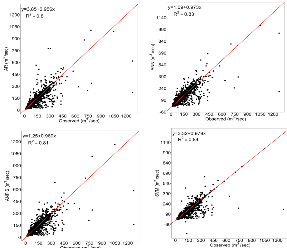
Figure 3.8. Daily streamflow observed vs estimated of the 1805 station. Red lines represent the best fit line
