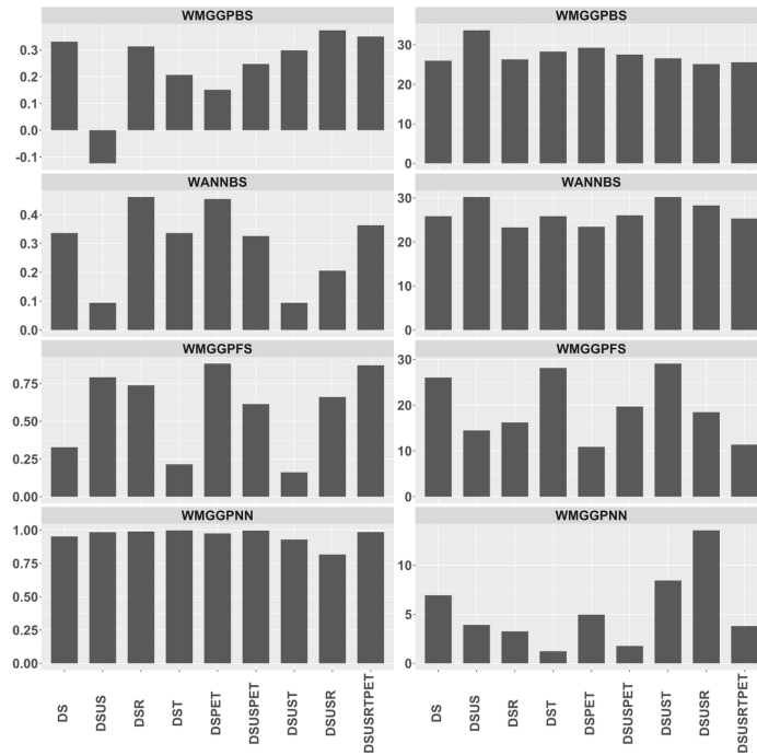
Figure 4.22. The performance of the models in forecasting the peak values. Left figures: R_p^2 , Right figures: RMSE_p
