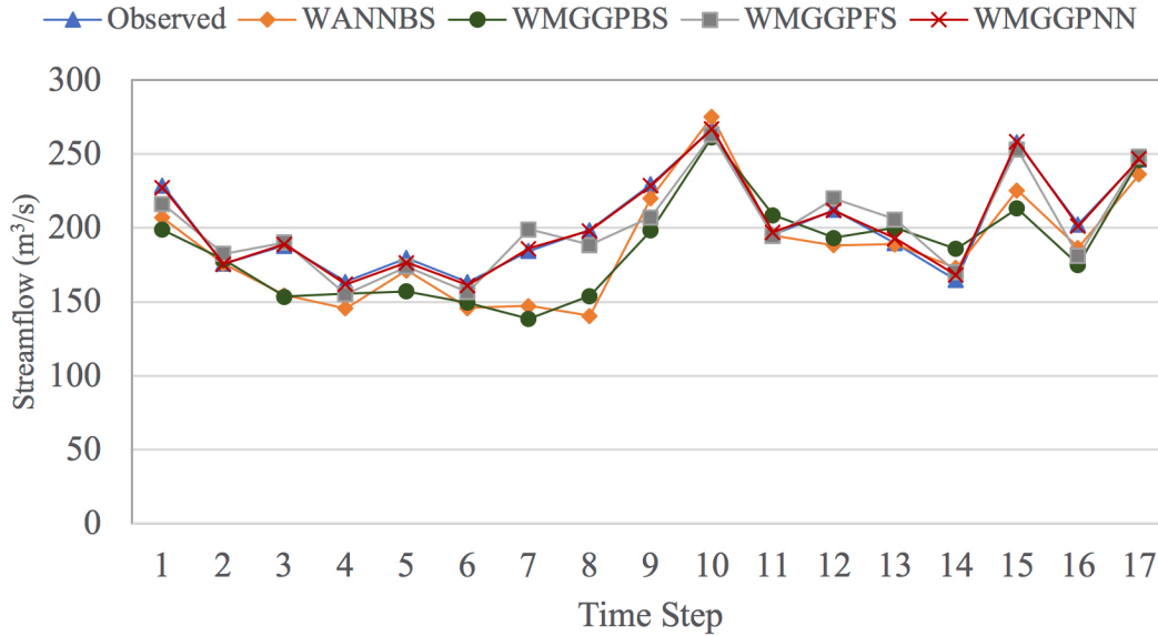
Figure 4.23. The observed and the predicted peak flows of the best-scale, full-scale and the proposed WMGGPNN model
