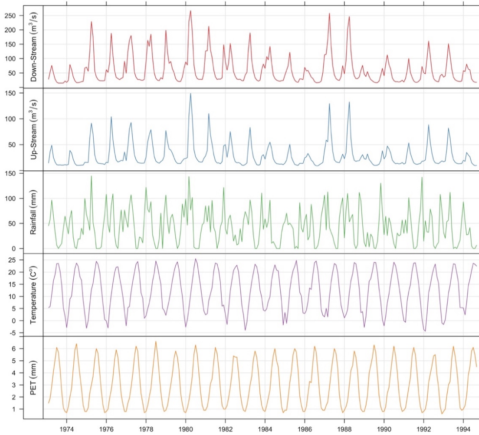
Figure 5.3. The time series of the variables used in the development of the models
