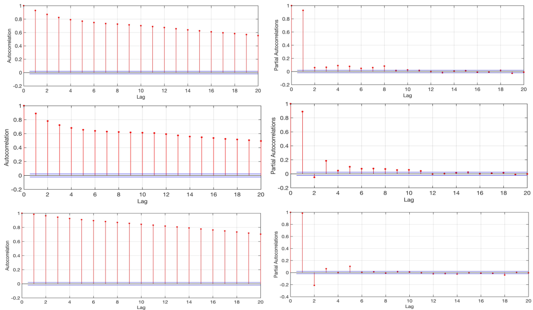
Figure 3.6. The Autocorrelation and partial autocorrelation functions of the three basins gage stations. from top to bottom: 1801, 1805 an 1822
