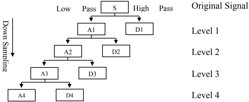
Figure 4.1. The discrete wavelet decomposition framework
