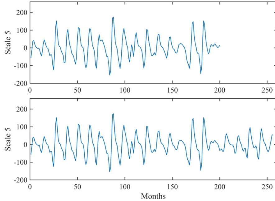
Figure 5.9. The coefficients of 5th scale of the downstream flow using CWT
