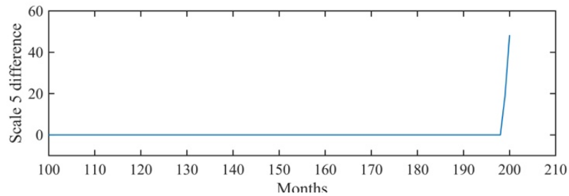
Figure 5.10. The difference between the first 200 months of coefficients of 5th scale of the downstream flow using CWT for 200 and 256 months
