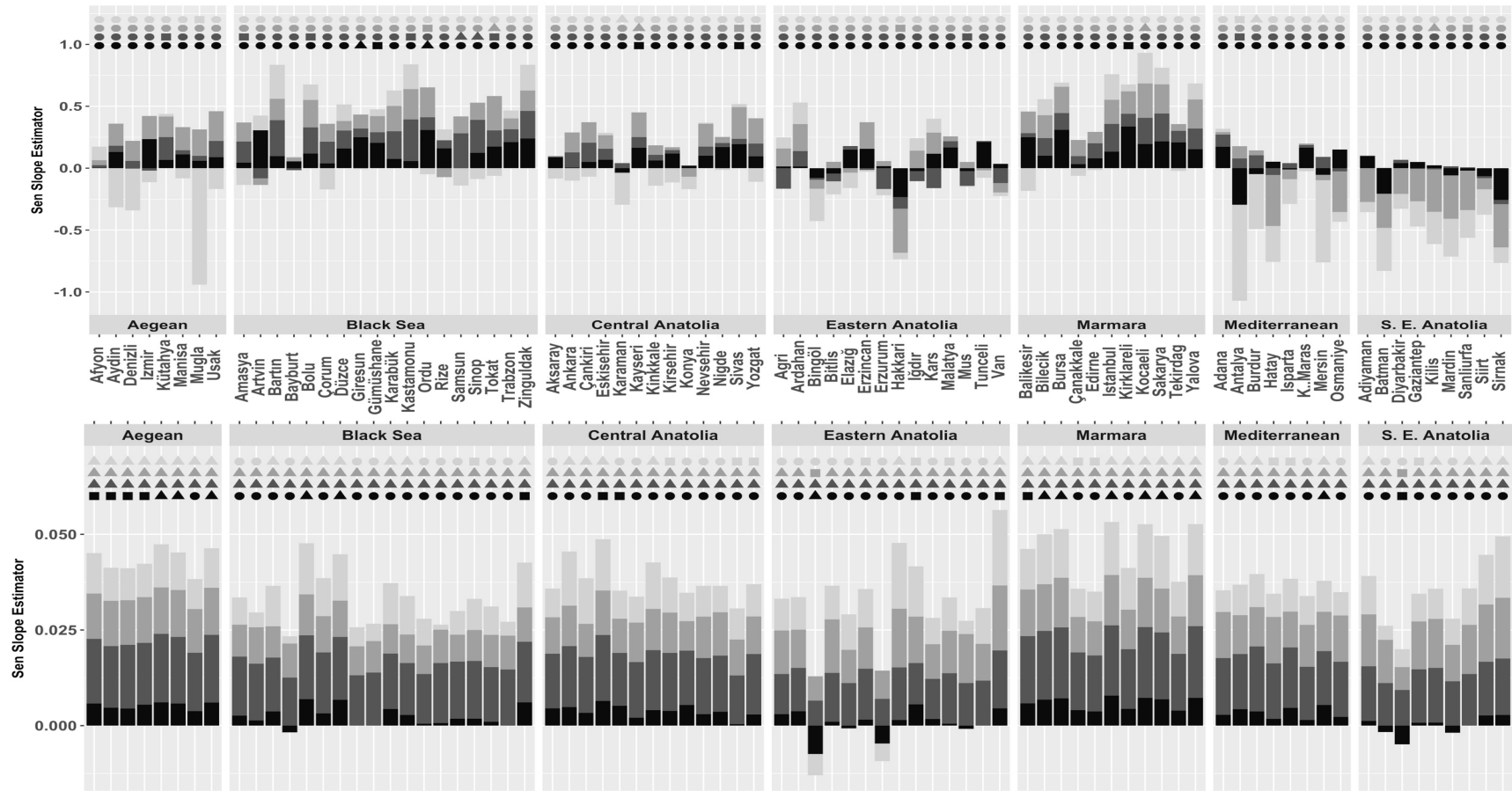
Figure 2.6. Seasonal Theil and Sen's Slope test values Top) Precipitation (mm/year), Bottom) Temperature (Co/year). Circle: Not significant, Square: significant at 0.1, Triangle: Significant at 0.05. Light to dark grey shades represents: Winter, Spring, Summer, and Autumn respectively
