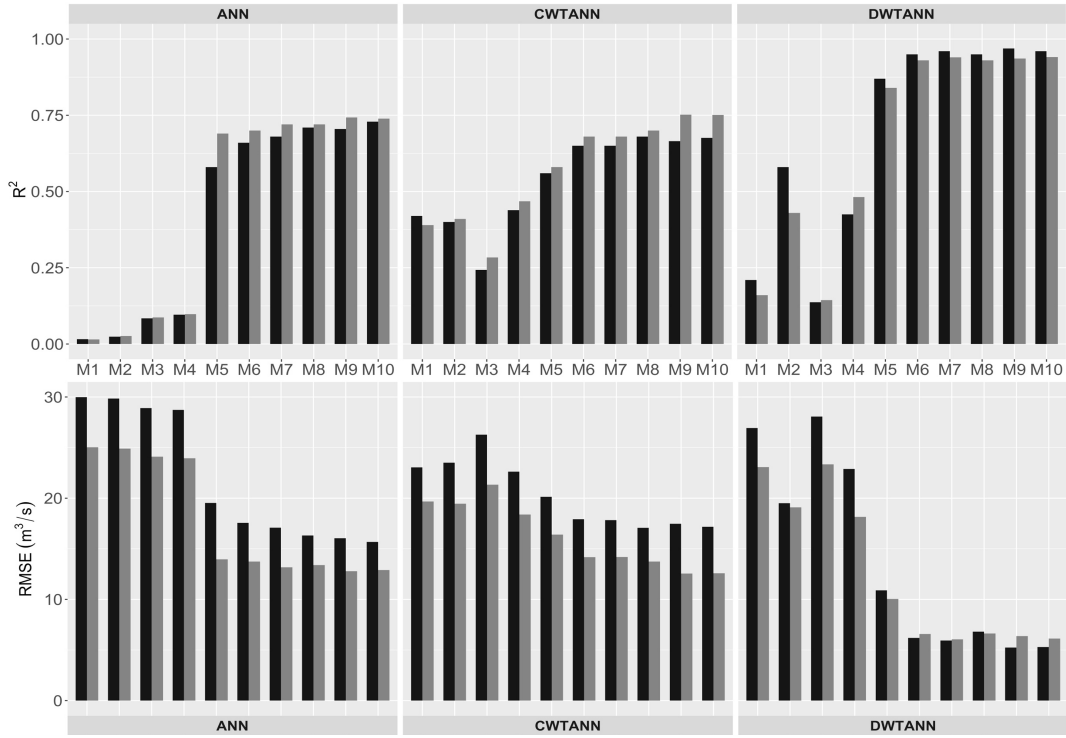
Figure 4.6. The R^2 and RMSE values of the three schematic layouts (ANN, CWTANN, and DWTANN)
