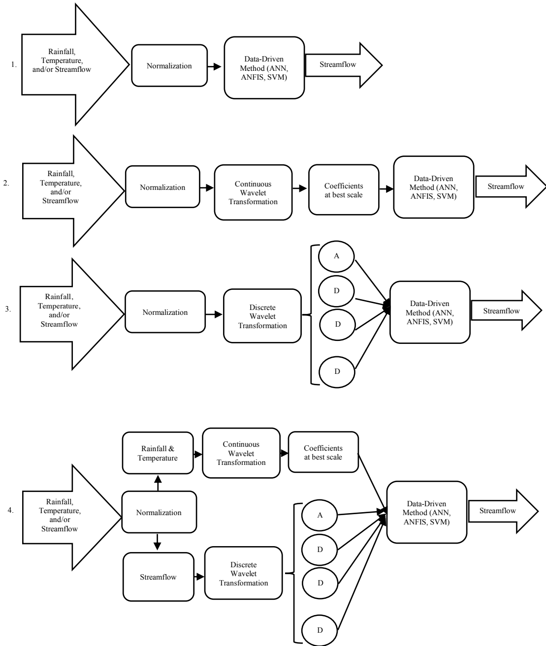
Figure 4.4. Schematic layouts of the applied models for forecasting streamflow
