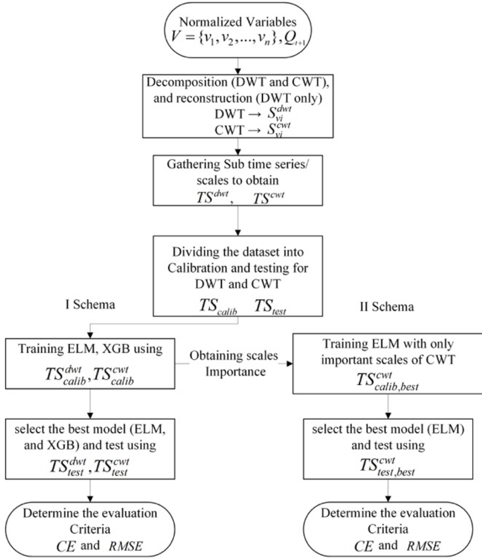
Figure 5.4. The framework of the hindcast experiment
