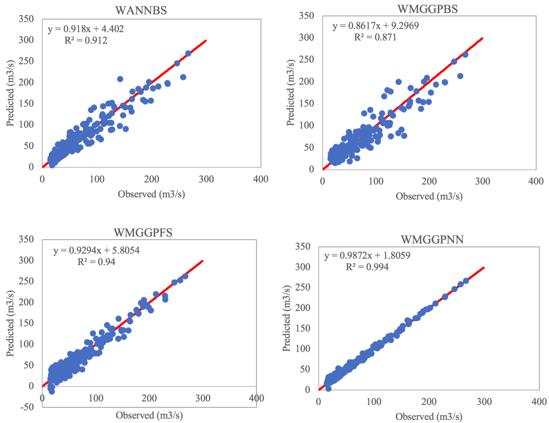
Figure 4.21. The observed vs predicted stream flows of the best-scale, full-scale and the proposed WMGGPNN model. Redline: the best fit
