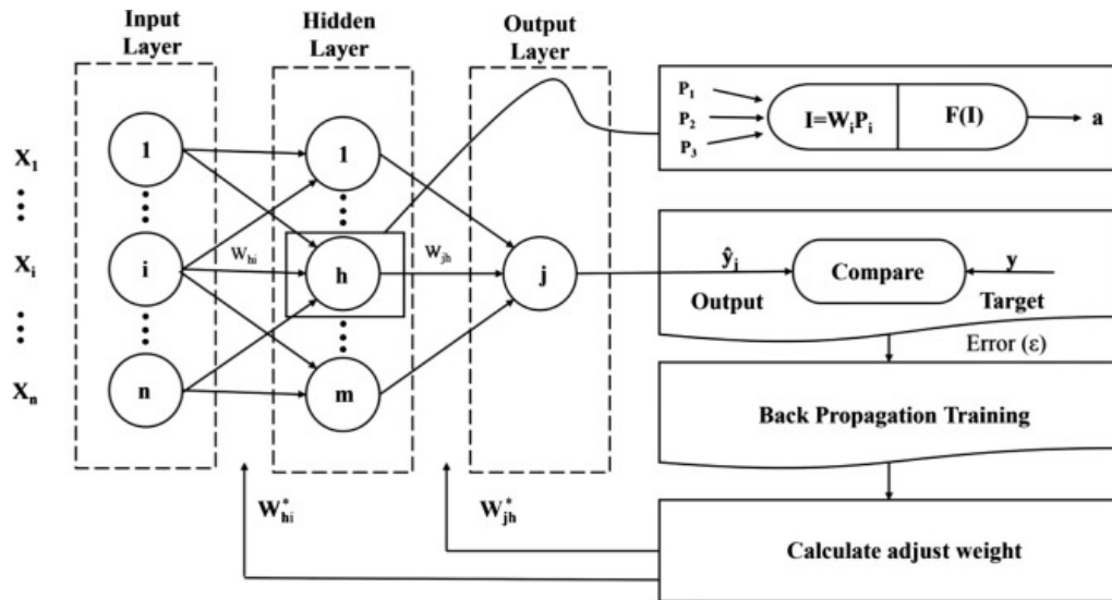
Figure 3.1. FFNN adapted from (Nourani 2017)
