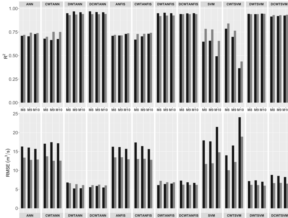
Figure 4.9. Comparison of R^2 and RMSE values between the schematic layouts of all DDMs for models M8, M9, and M10
