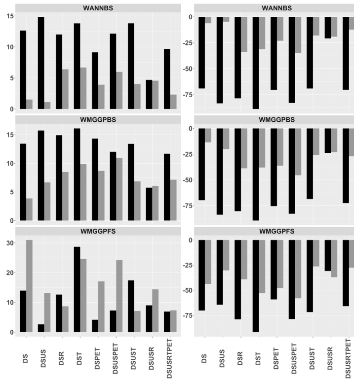
Figure 4.20. Percentage of change in R^2 (left figures), and RMSE (right figures) relatively to the proposed model WMGGPNN. Black colour: Training subset, Grey Colour: Validation subset
