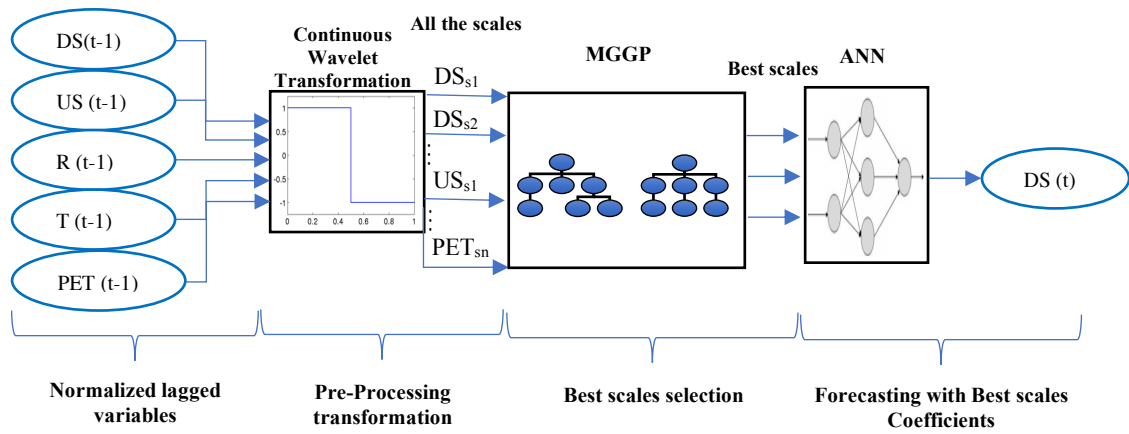
Figure 4.14. Schematic layout of the proposed model
