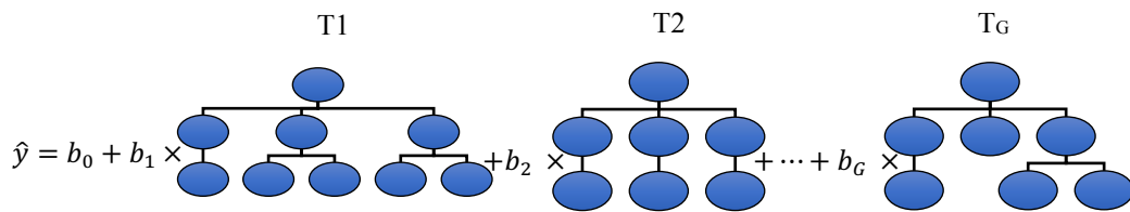
Figure 4.13. Multi Gene Genetic Programming (Symbolic Regression)
