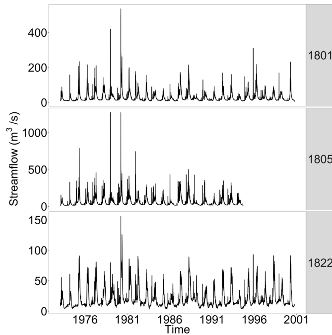
Figure 3.5. Time series of the Streamflow
