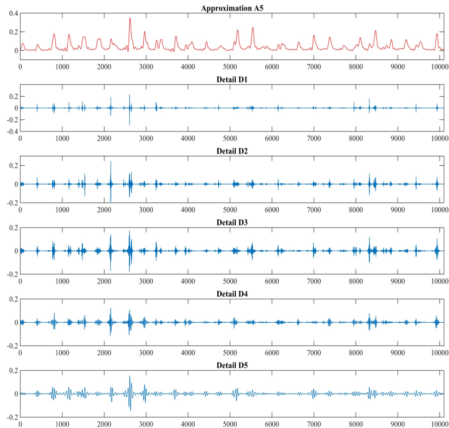
Figure 4.5. the decomposition of the daily streamflow using “dmey” function with 5 levels
