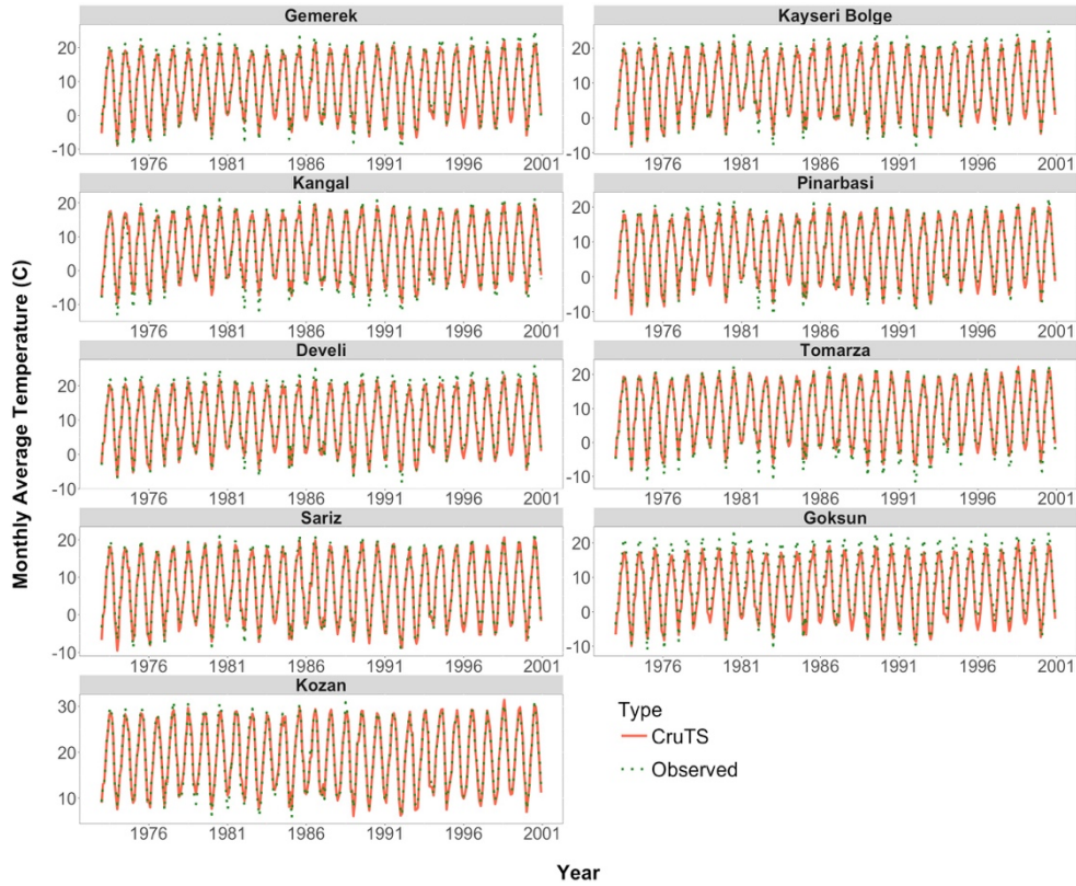
Figure 1.9. Time series plot of the monthly average temperature obtained from CruTS and Observed data for the period 1973 - 2000
