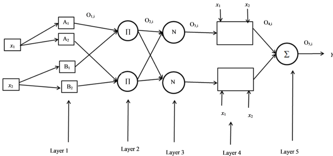
Figure 3.2. ANFIS framework
