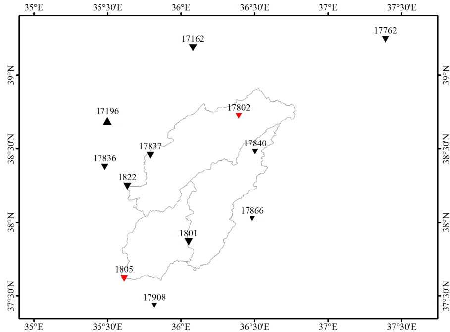
Figure 2.11. Spatial distribution of the stations with the annual trend. The size of the triangle represents the normalized magnitude of the trend. The up-pointing triangle: positive trend, the down pointing triangle: negative trend. Black: Not significant, Red: Significant at \alpha=0.1
