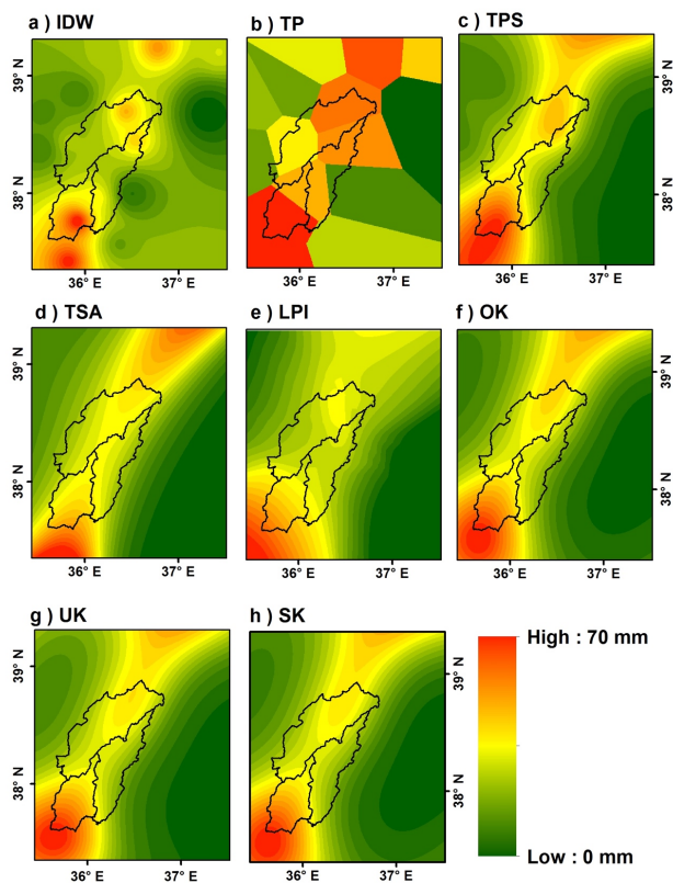
Figure 1.2. Examples of interpolated maps of monthly total precipitation (in mm) for each of the 8 interpolation methods. The month chosen as an example is June 1989
