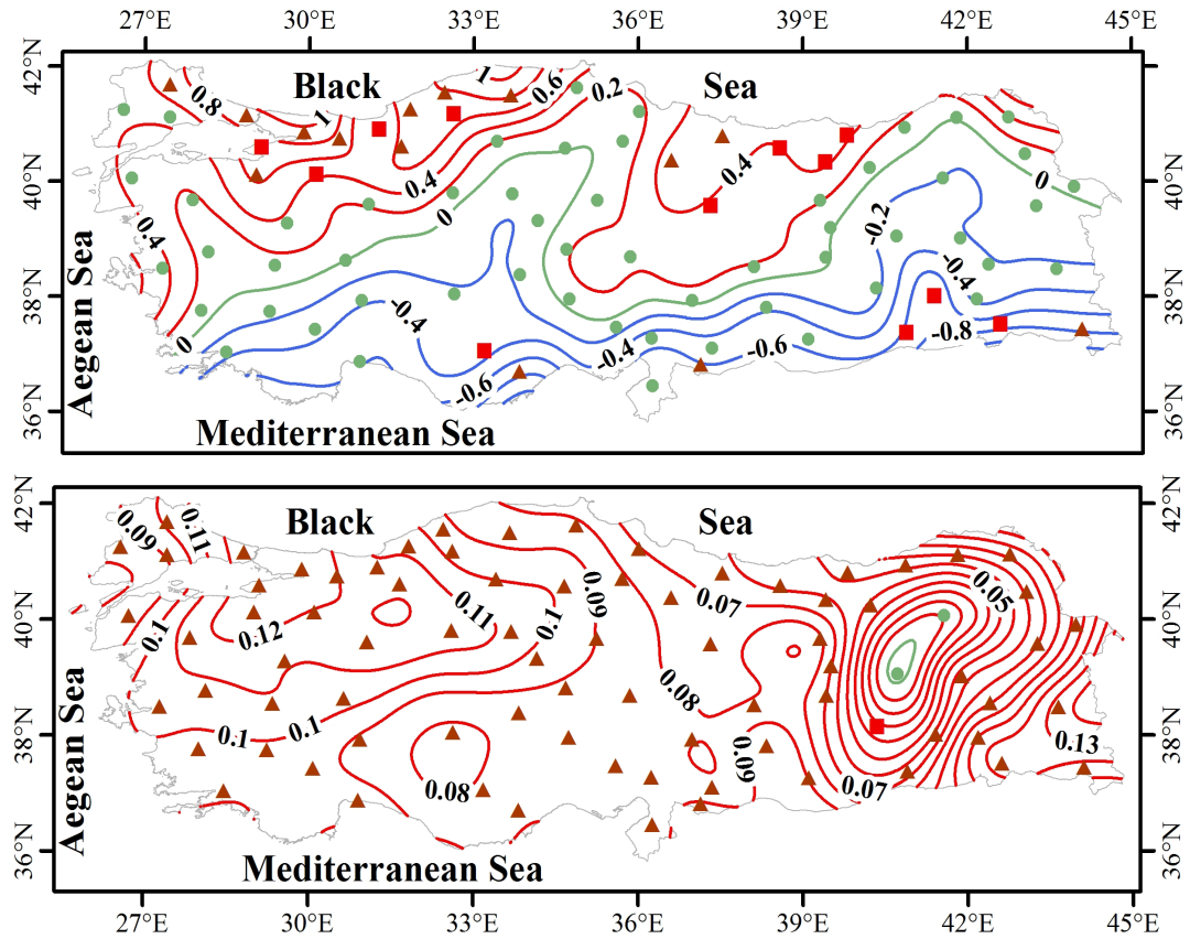
Figure 2.5. Contour lines for the spatial distribution of the Annual Theil and Sen's Slope test values Top) Precipitation (mm/year), Bottom) Temperature (Co/decade)
