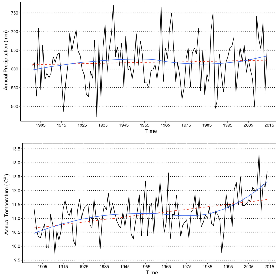
Figure 2.3. The time series of Turkey's mean of the total annual precipitation (Top) and the average annual temperature (bottom). Solid Line: LOWESS regression, Dashed Line: Simple Linear Regression. For Precipitation(Temperature), Insignificant (Significant) trend with 0.11 mm/year (0.88 C°/Century) Theil and Sen's Slope test value and change year 1934 (1993)
