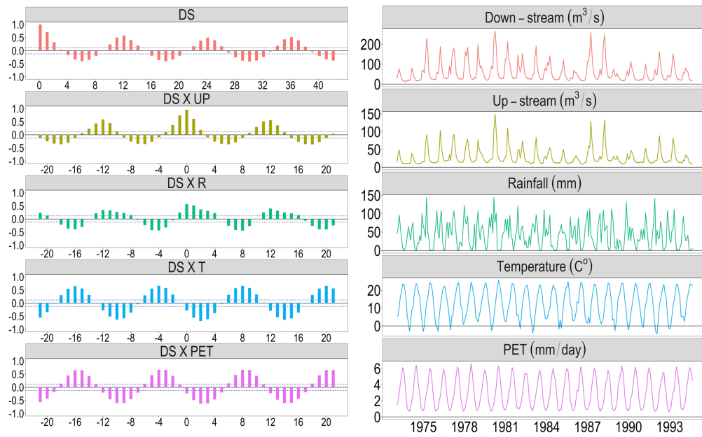
Figure 4.16. Time series of the monthly variables (Right figures) and the ACF of the downstream and the CCF of the downstream and each variable (Left figures)
