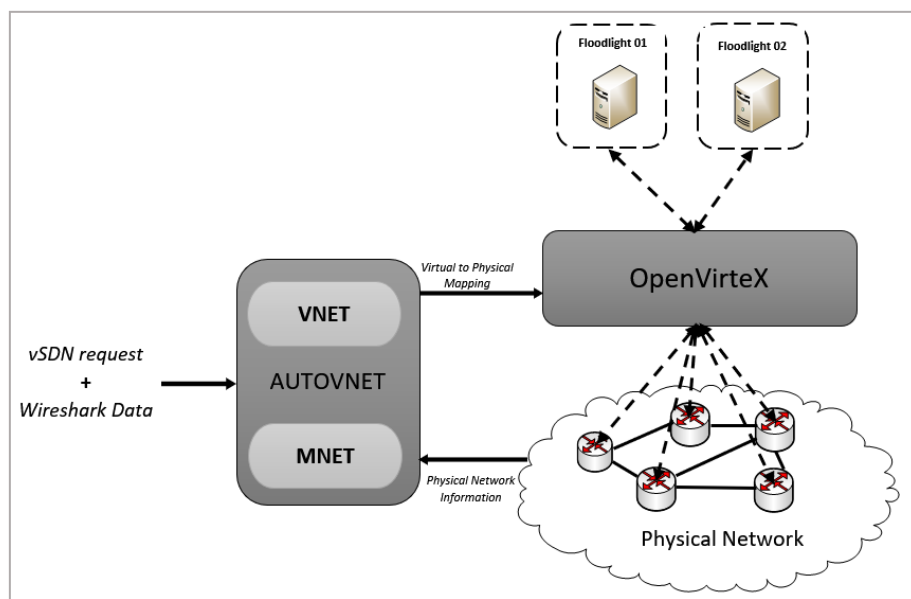
Figure 4.1. AUTOVNET system architecture
