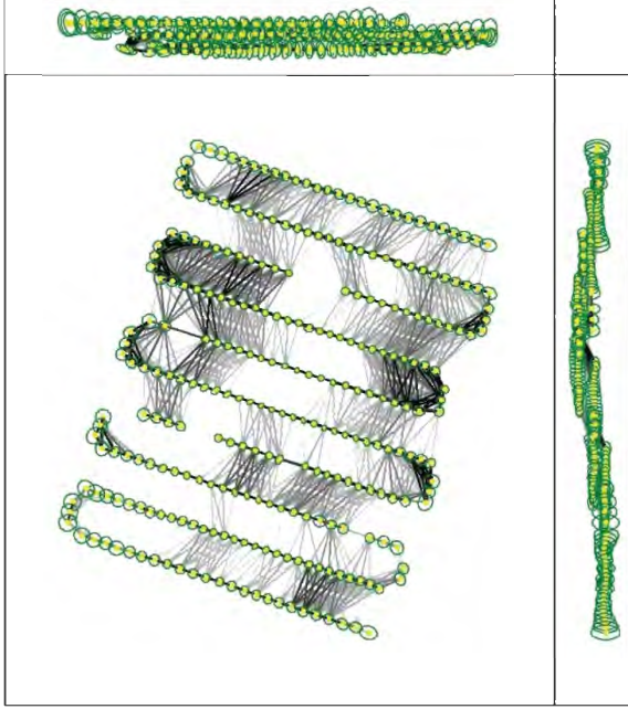
Figure 5: Computed image positions and the links between matched images. The darkness of the links indicates the number of matched 2D keypoints between the images. Bright links indicate weak links and require manual matches. Dark green ellipses indicate the relative camera position uncertainty of the bundle block adjustment result.
