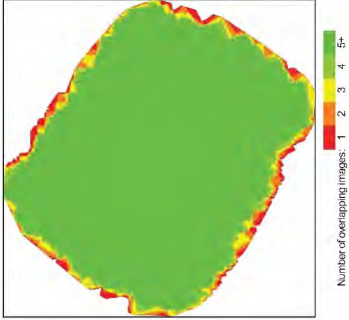
Figure 4: Number of overlapping images computed for each pixel of the orthomosaic. Red and yellow areas indicate low overlap, while green areas indicate high overlap. Good quality results will be generated as long as the number of keypoint matches is also sufficient for these areas (see Figure 5 for keypoint matches).
