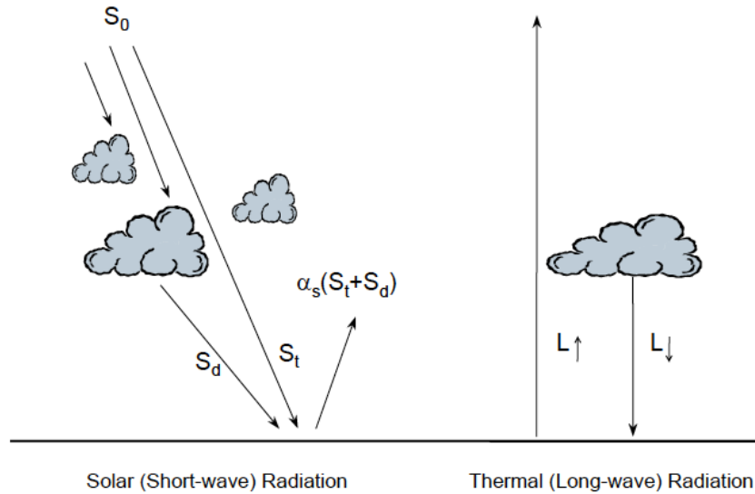
Figure 2.1. Radiation Classification (Finch & Hall, 2001)
