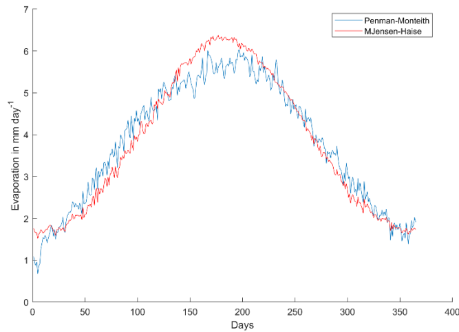
Figure 4.12. Variation of evaporation rates for daily time step estimated using Modified Jensen-Haise equation
