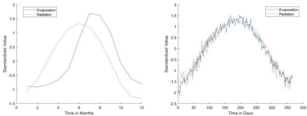
Figure 4.5. Total solar radiation effect on evaporation at different time-scales (yearly values are averaged to monthly values for the period 2000-2013)
