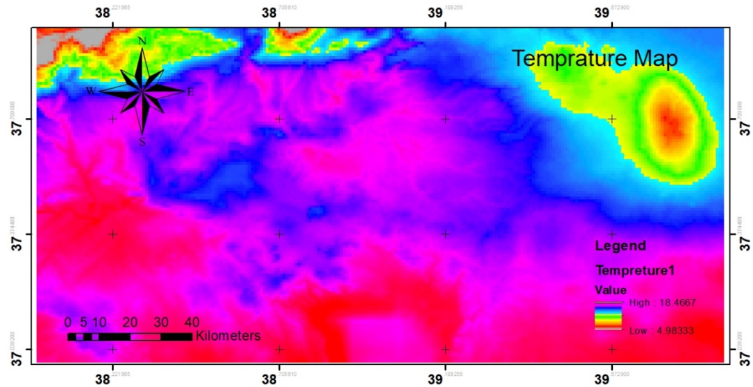
Figure 4.1. Temperature record for the Bozova district and relative area for the year 1979-2010
