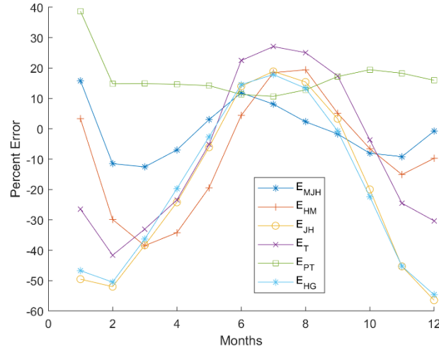
Figure 4.11. Variation of percentage error in evaporation estimates using Hargreaves, Hamon, Jensen-Haise, Priestly-Taylor, Turc and Modified Jensen-Haise methods
