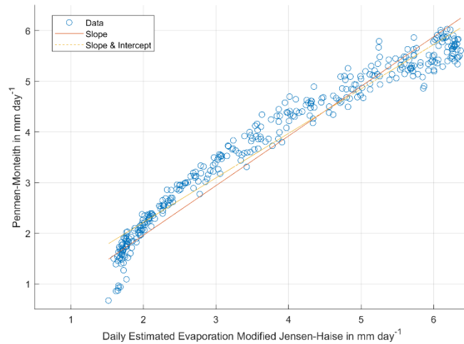
Figure 4.16. Comparison of EPM with estimated ET for the Modified Jensen-Haise equation.
