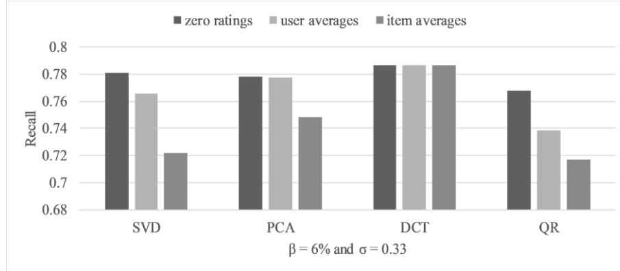
Figure 4.1. Recall with different default values
