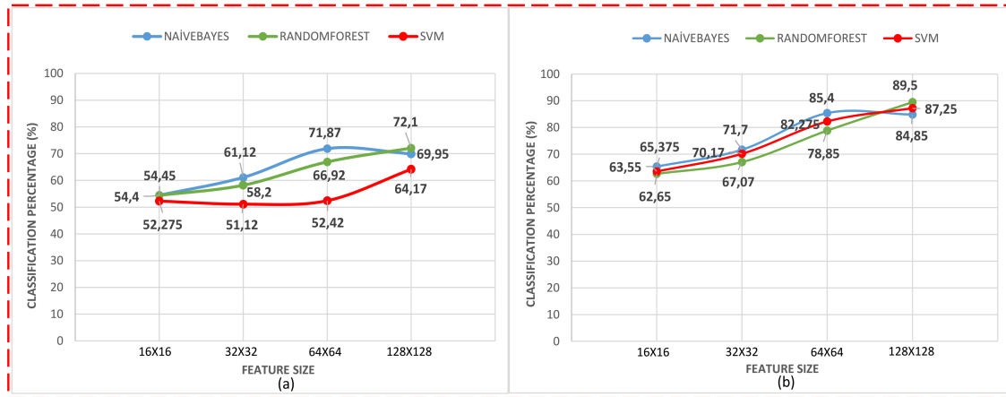
Figure 2.8. Classification results using LBP at various feature sizes for (a) IR and (b) VL images.
