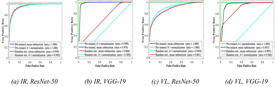
Figure 2.23. Receiver operating characteristic (ROC) curves of the end-to-end classification method. The legend is in the order of decreasing area under the curve. Note that the curves of the best performing methods overlap and occlude each other in some Figures.
