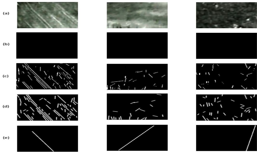
Figure 2.27. In CNN's stage analysis, maximum result is found in ResNet-50 (mean subtraction process) architecture, IR image dataset, False positive results compared to other methods. Line detection results: (a) IR images (with powerlines, incorrectly detected with CNN stage analysis), (b) Ground Truth (c) EDLines, (d) LSD and (e) HT. Edge/line detection methods incorrect.
