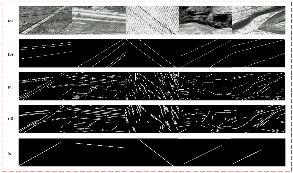
Figure 2.16. Edge/Line detection results : (a) IR images (with powerlines, correctly detected by our method), (b) Ground Truth of (a), (c) EDLines (d) LSD and (e) HT. Edge/line detection methods incorrect.
