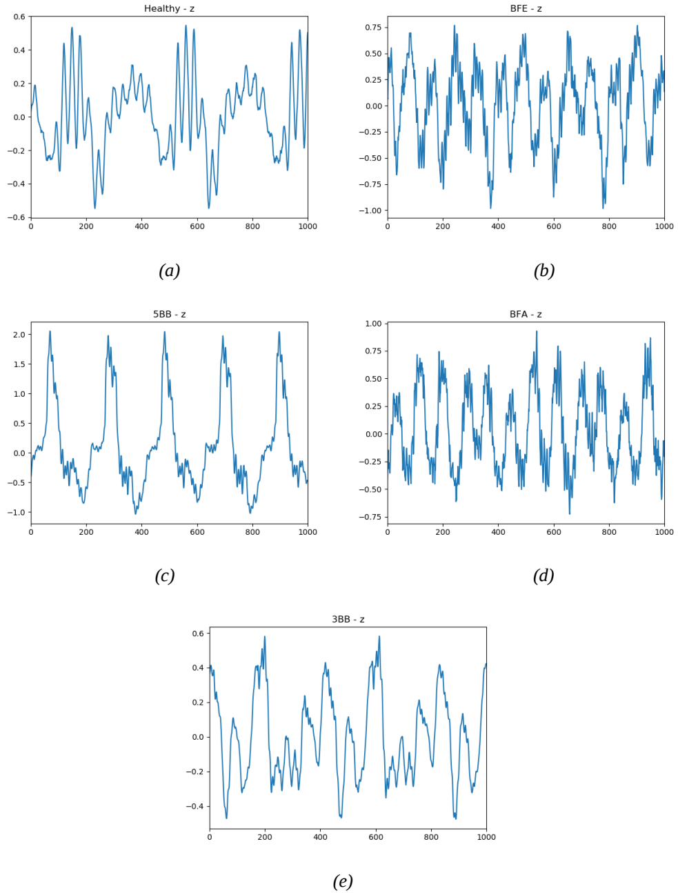
Figure 4.4. The first 1000 vibration data from z- axis of (a) Healthy (b) BFE (c) 5BB (d) BFA (e) 3BB faulty induction motor under 4.1 Amperes
